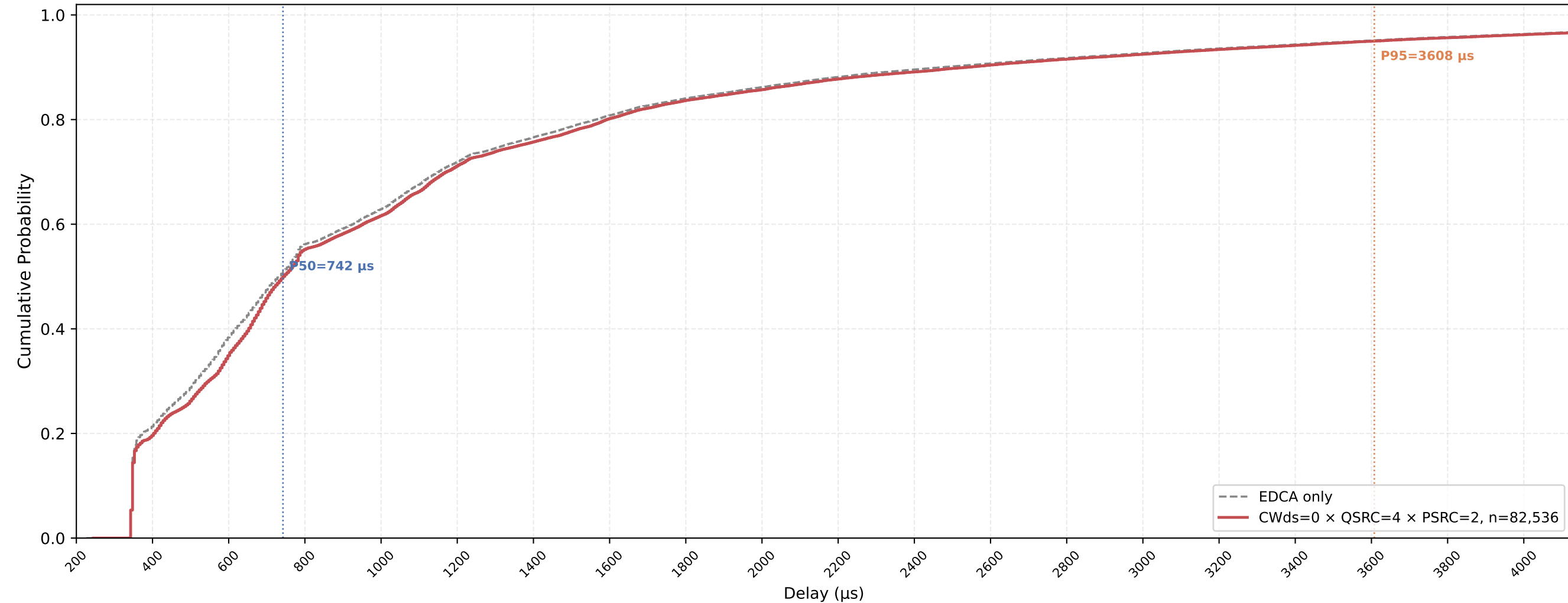
Legacy STA VO Delay CDF — CWds=0 × QSRC=4 × PSRC=2 nSta=30, nPedca=15, 0.5Mbps, avg of 10 runs
