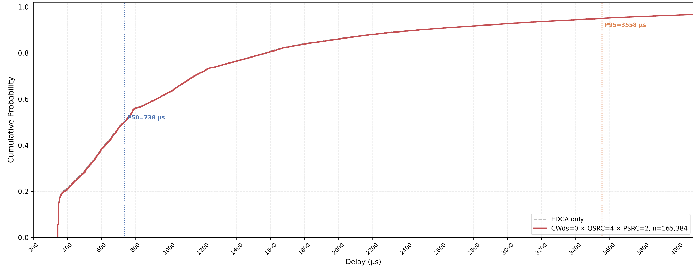
VO (all STAs) Delay CDF — CWds=0 × QSRC=4 × PSRC=2 nSta=30, nPedca=5, 0.5Mbps, avg of 10 runs
