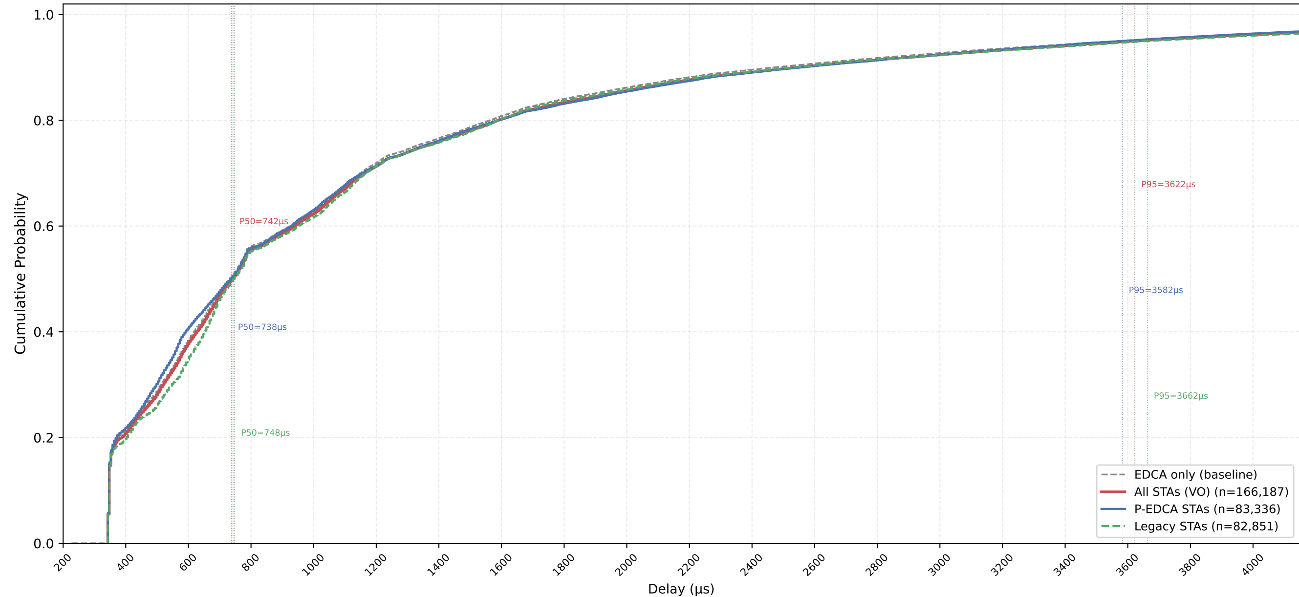
VO Delay CDF — P-EDCA / Legacy / All | CWds=0 × QSRC=4 × PSRC=3 nSta=30, nPedca=15/30, 0.5Mbps, avg of 10 runs
