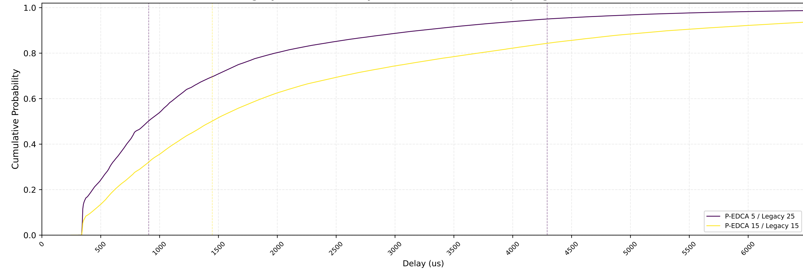
Legacy EDCA STAs Delay CDF — nSta=30, 0.5Mbps, avg of 10 runs
