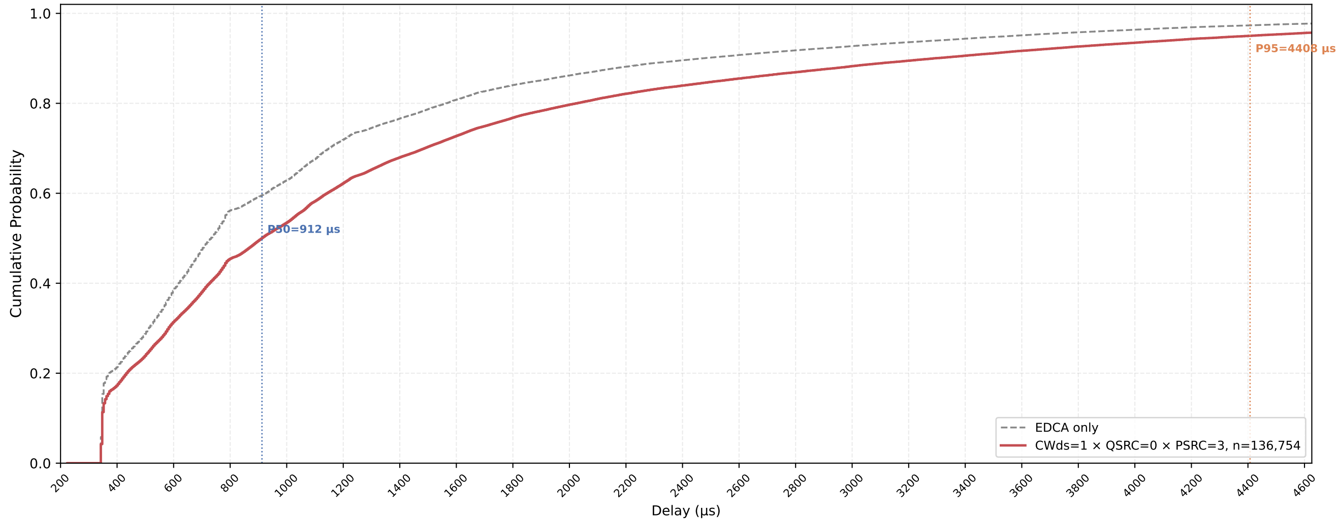
Legacy STA VO Delay CDF — CWds=1 × QSRC=0 × PSRC=3 nSta=30, nPedca=5, 0.5Mbps, avg of 10 runs
