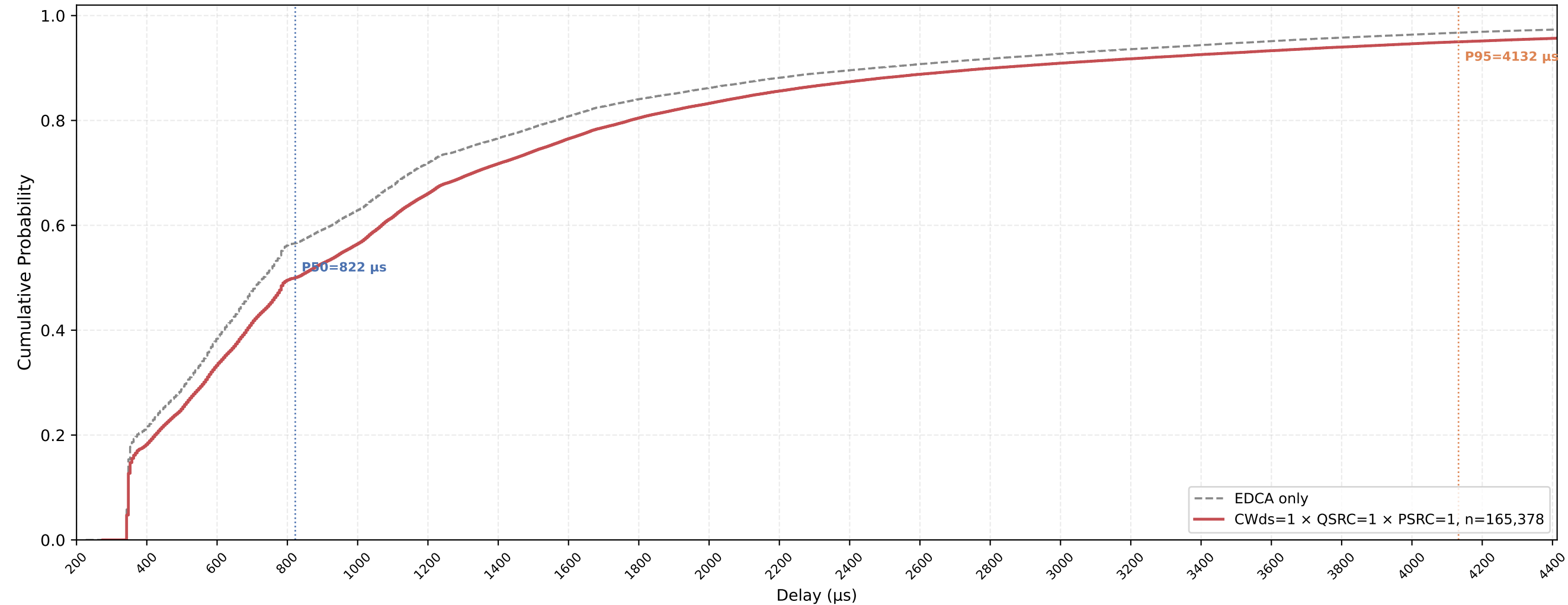
VO (all STAs) Delay CDF — CWds=1 × QSRC=1 × PSRC=1 nSta=30, nPedca=15, 0.5Mbps, avg of 10 runs
