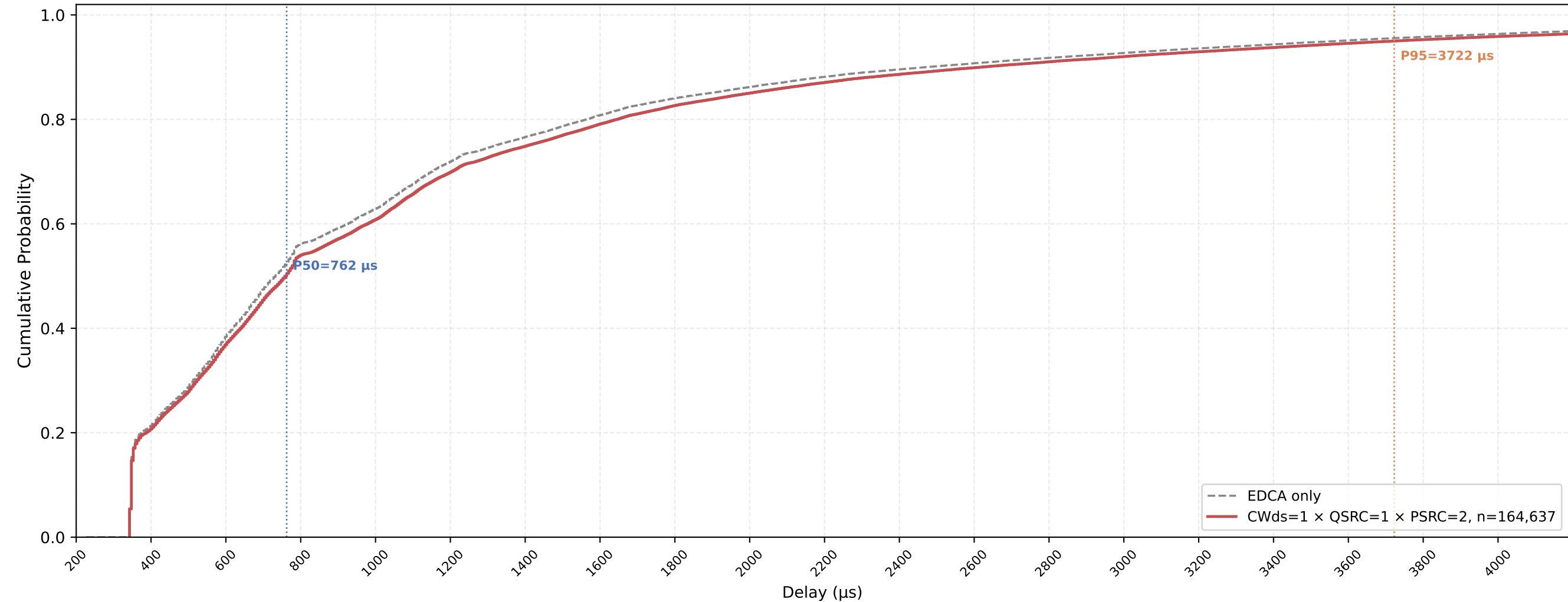
VO (all STAs) Delay CDF — CWds=1 × QSRC=1 × PSRC=2 nSta=30, nPedca=5, 0.5Mbps, avg of 10 runs
