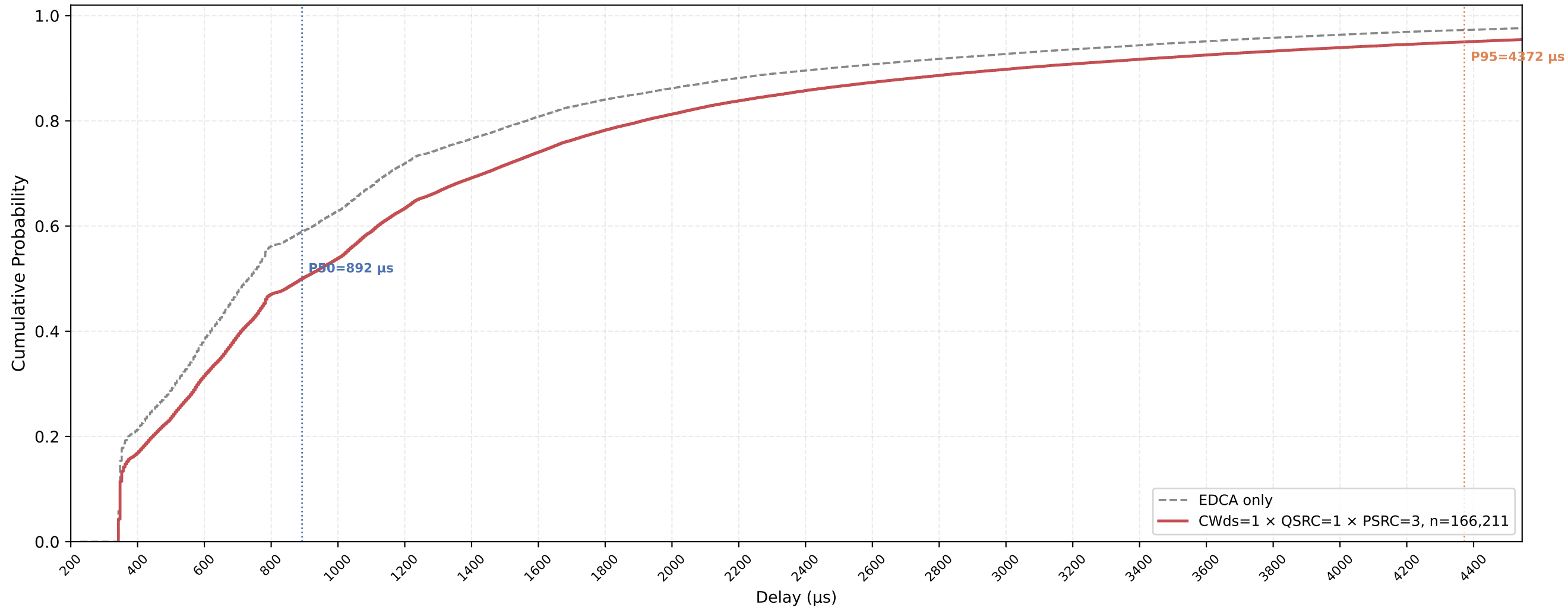
VO (all STAs) Delay CDF — CWds=1 × QSRC=1 × PSRC=3 nSta=30, nPedca=15, 0.5Mbps, avg of 10 runs
