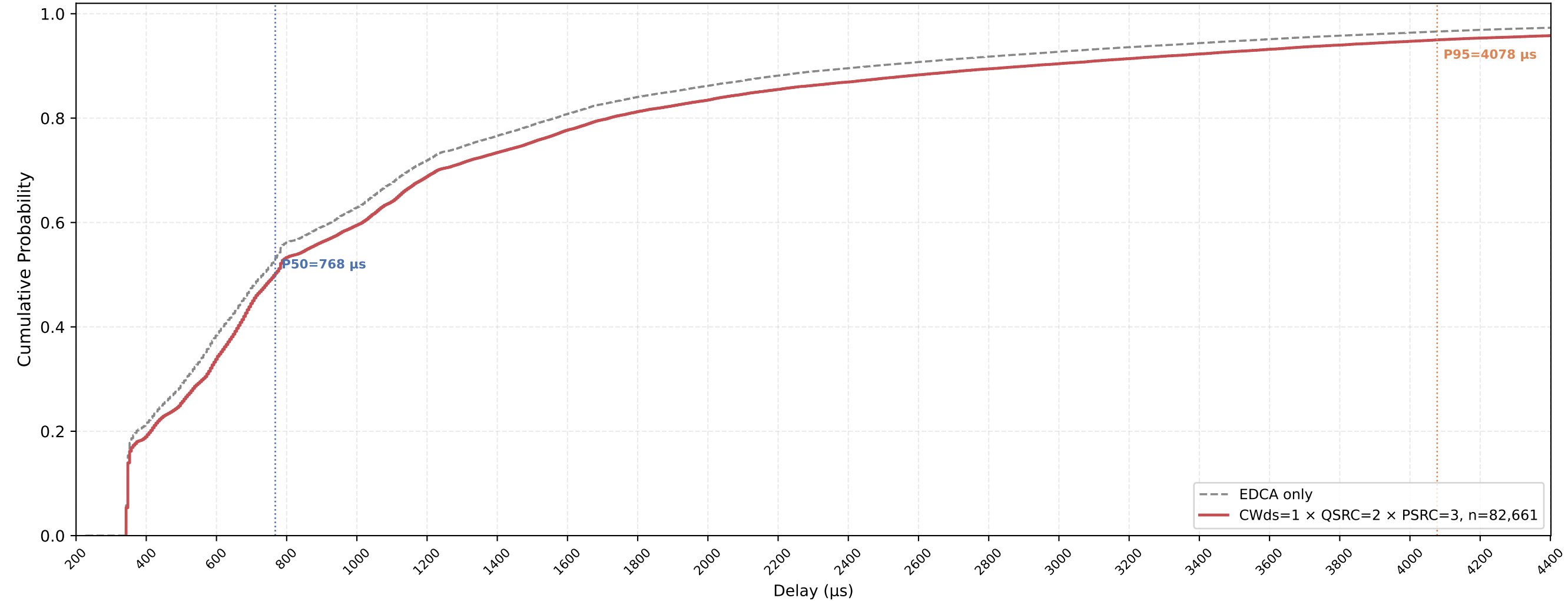
Legacy STA VO Delay CDF — CWds=1 × QSRC=2 × PSRC=3 nSta=30, nPedca=15, 0.5Mbps, avg of 10 runs
