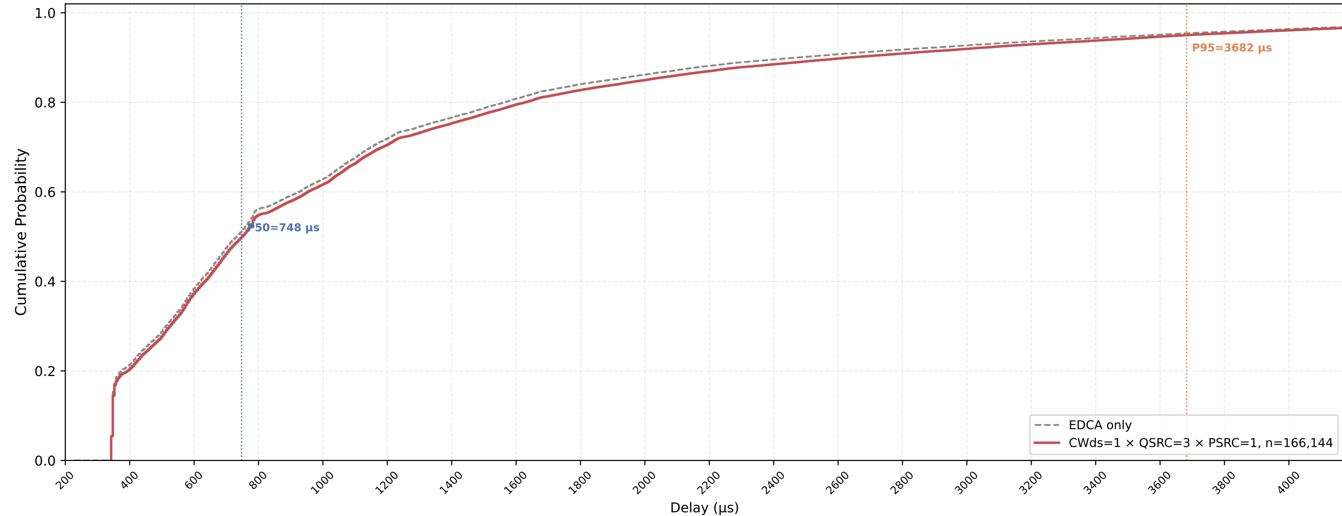
VO (all STAs) Delay CDF — CWds=1 × QSRC=3 × PSRC=1 nSta=30, nPedca=15, 0.5Mbps, avg of 10 runs
