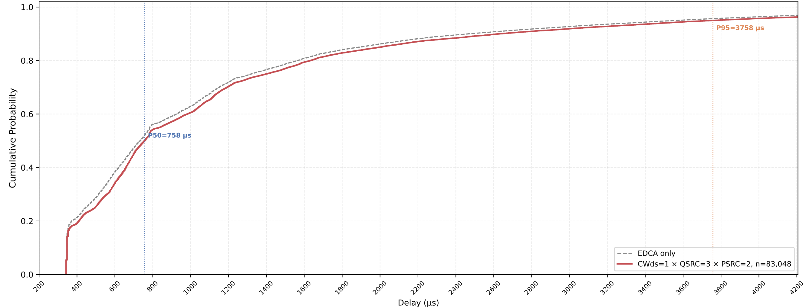
Legacy STA VO Delay CDF — CWds=1 × QSRC=3 × PSRC=2 nSta=30, nPedca=15, 0.5Mbps, avg of 10 runs
