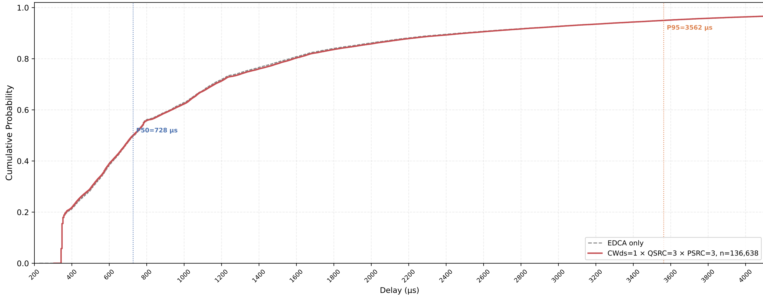
Legacy STA VO Delay CDF — CWds=1 × QSRC=3 × PSRC=3 nSta=30, nPedca=5, 0.5Mbps, avg of 10 runs
