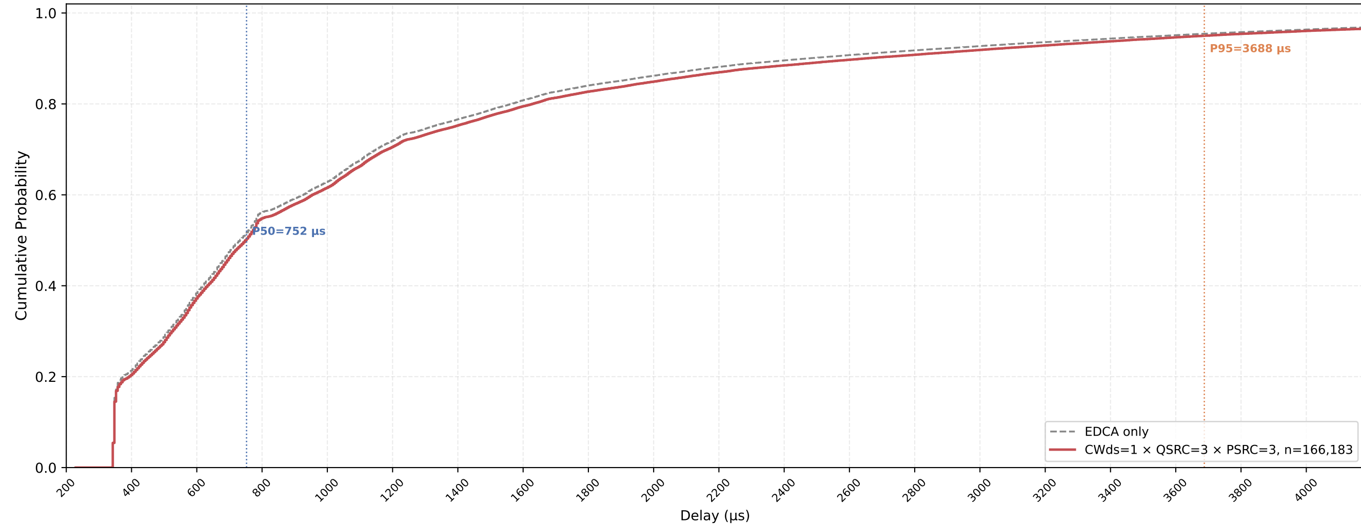
VO (all STAs) Delay CDF — CWds=1 × QSRC=3 × PSRC=3 nSta=30, nPedca=15, 0.5Mbps, avg of 10 runs
