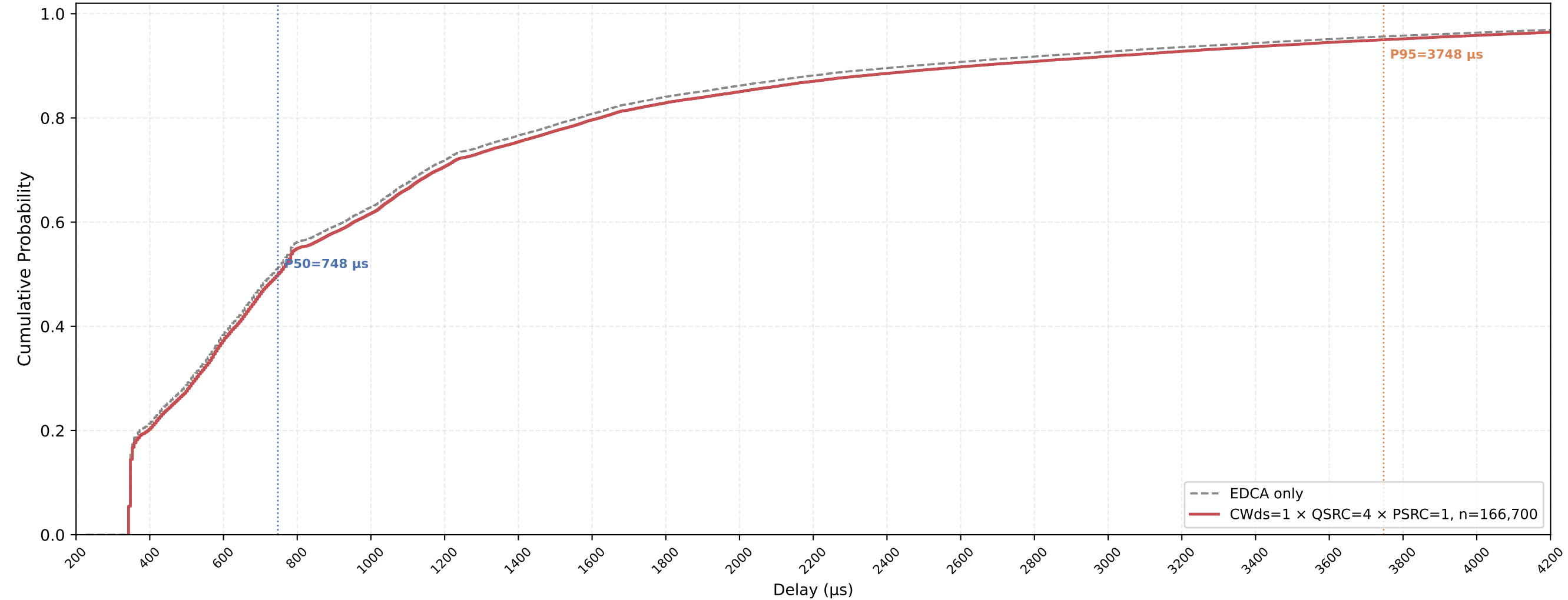
P-EDCA STA VO Delay CDF — CWds=1 × QSRC=4 × PSRC=1 nSta=30, nPedca=30, 0.5Mbps, avg of 10 runs
