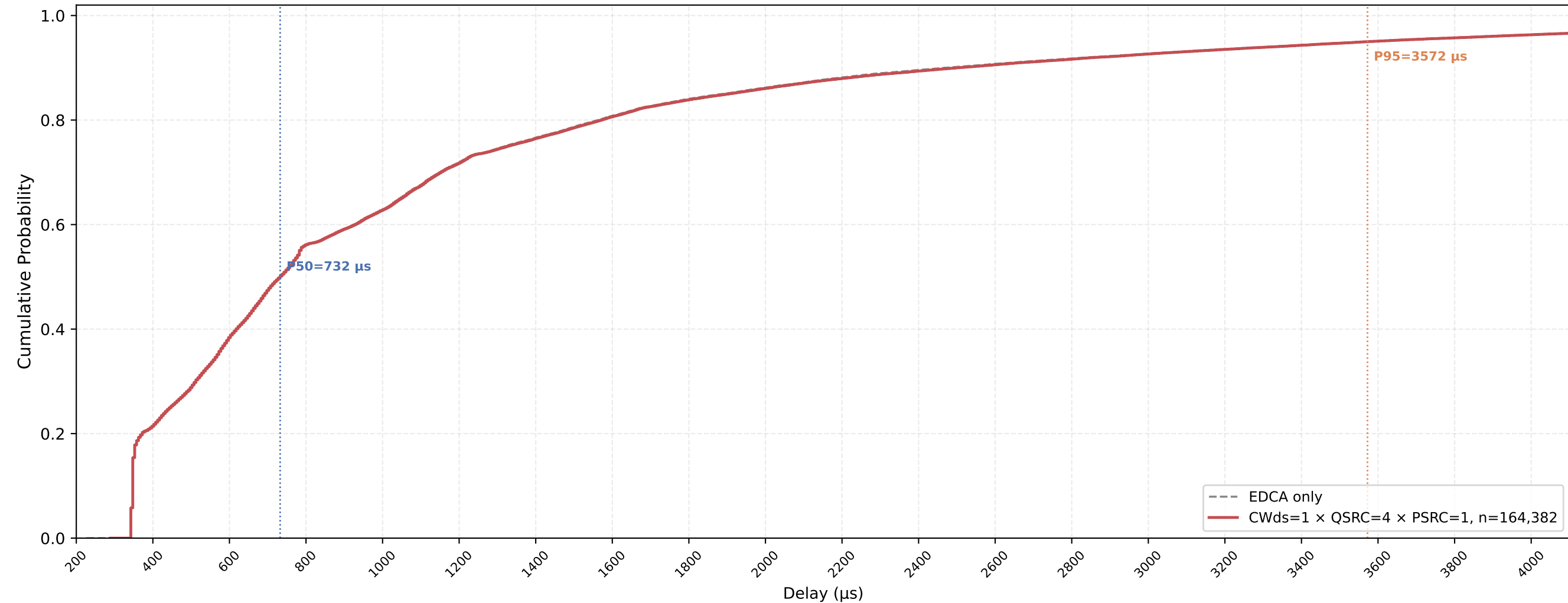
VO (all STAs) Delay CDF — CWds=1 × QSRC=4 × PSRC=1 nSta=30, nPedca=5, 0.5Mbps, avg of 10 runs
