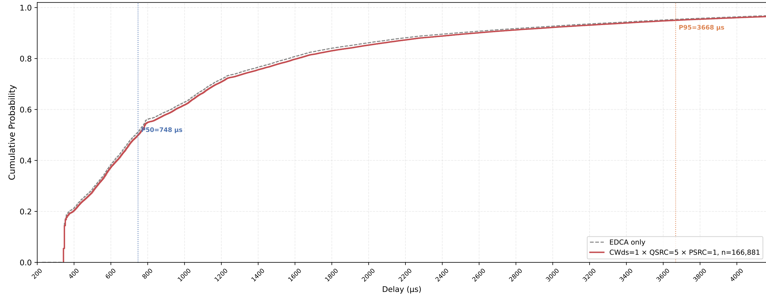
P-EDCA STA VO Delay CDF — CWds=1 × QSRC=5 × PSRC=1 nSta=30, nPedca=30, 0.5Mbps, avg of 10 runs
