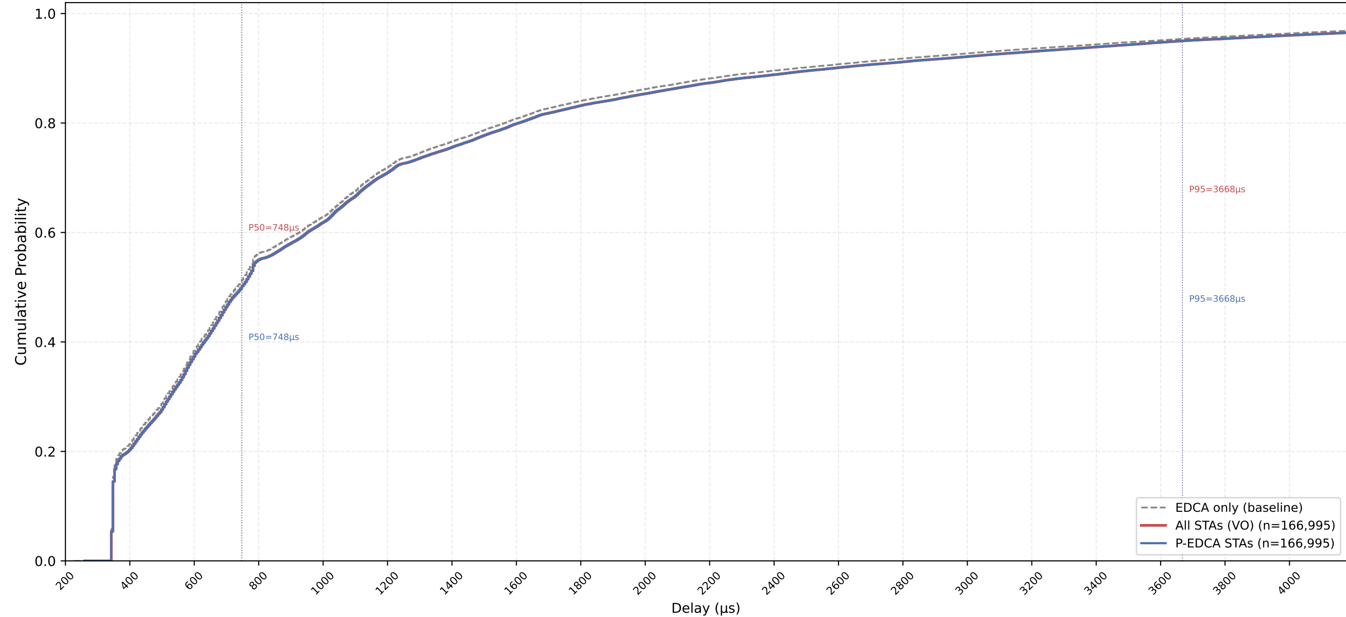
VO Delay CDF — P-EDCA / Legacy / All | CWds=1 × QSRC=5 × PSRC=2 nSta=30, nPedca=30/30, 0.5Mbps, avg of 10 runs
