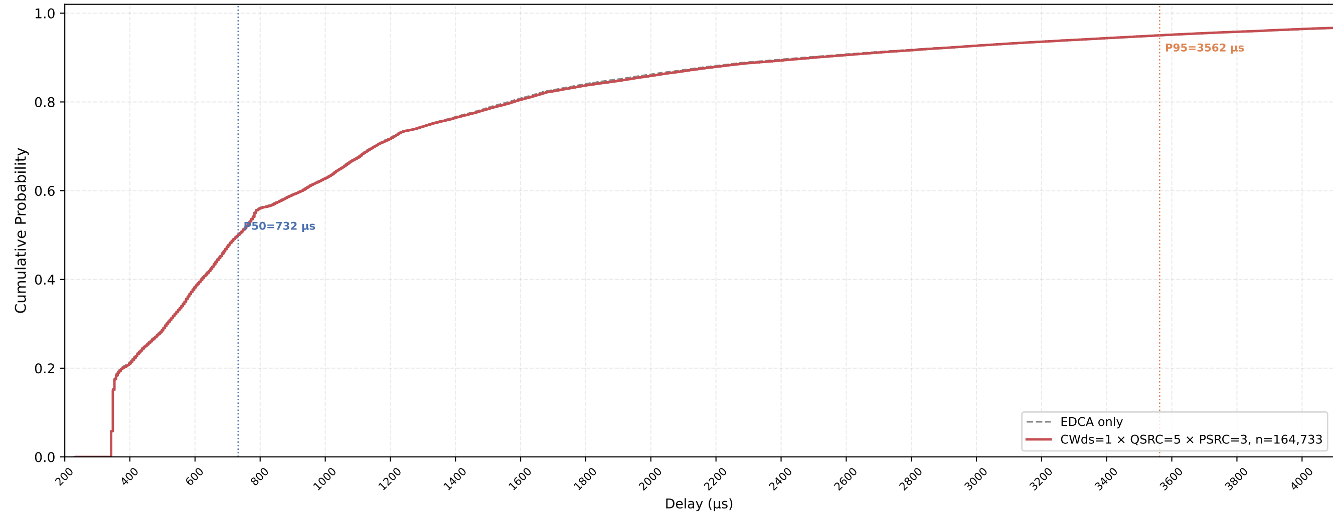
VO (all STAs) Delay CDF — CWds=1 × QSRC=5 × PSRC=3 nSta=30, nPedca=5, 0.5Mbps, avg of 10 runs
