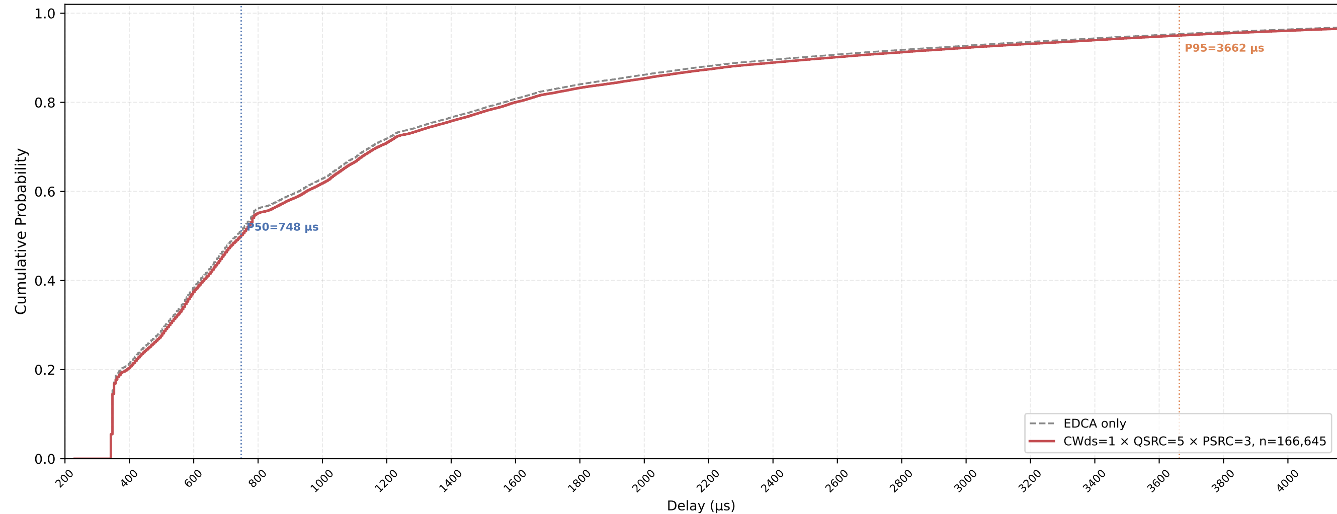
VO (all STAs) Delay CDF — CWds=1 × QSRC=5 × PSRC=3 nSta=30, nPedca=30, 0.5Mbps, avg of 10 runs
