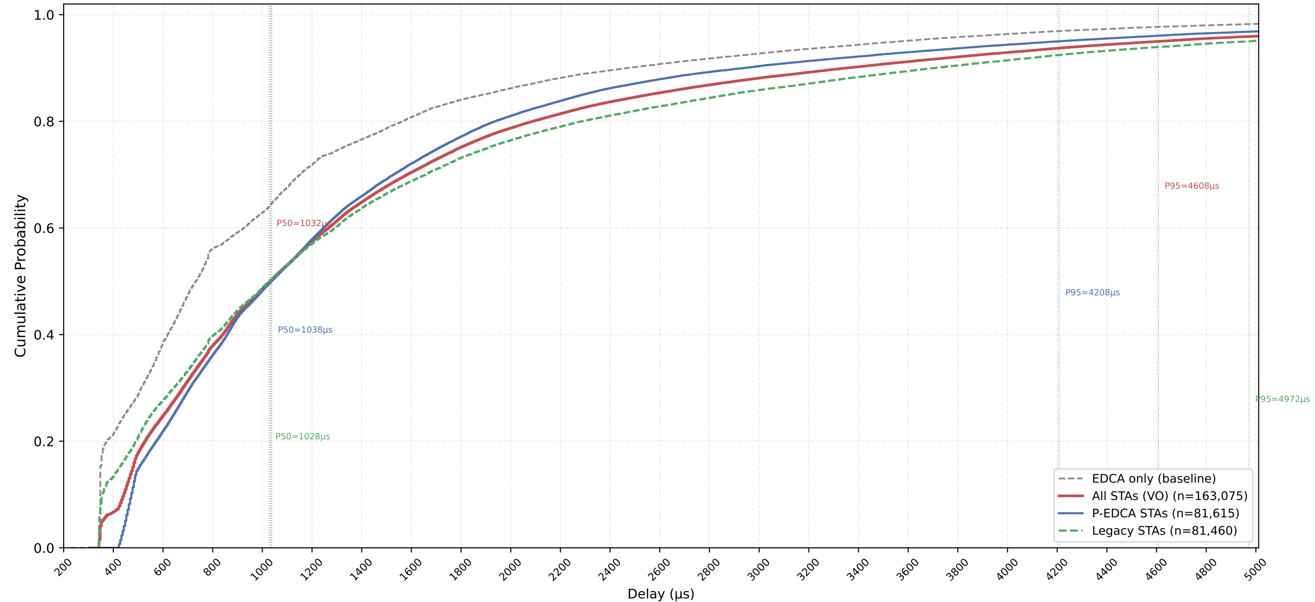
VO Delay CDF — P-EDCA / Legacy / All | CWds=0 × QSRC=0 × PSRC=1 nSta=30, nPedca=15/30, 0.5Mbps, avg of 10 runs
