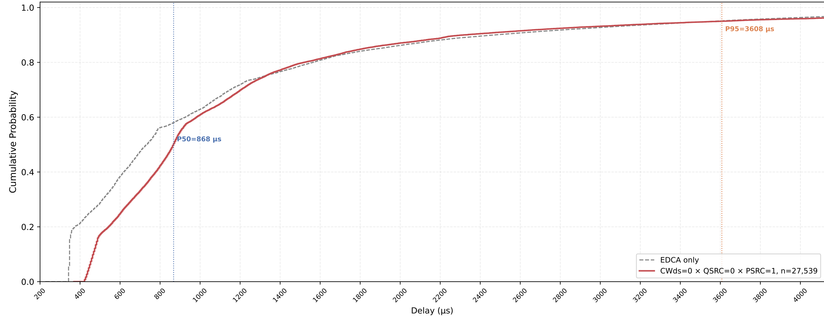
P-EDCA STA VO Delay CDF — CWds=0 × QSRC=0 × PSRC=1 nSta=30, nPedca=5, 0.5Mbps, avg of 10 runs
