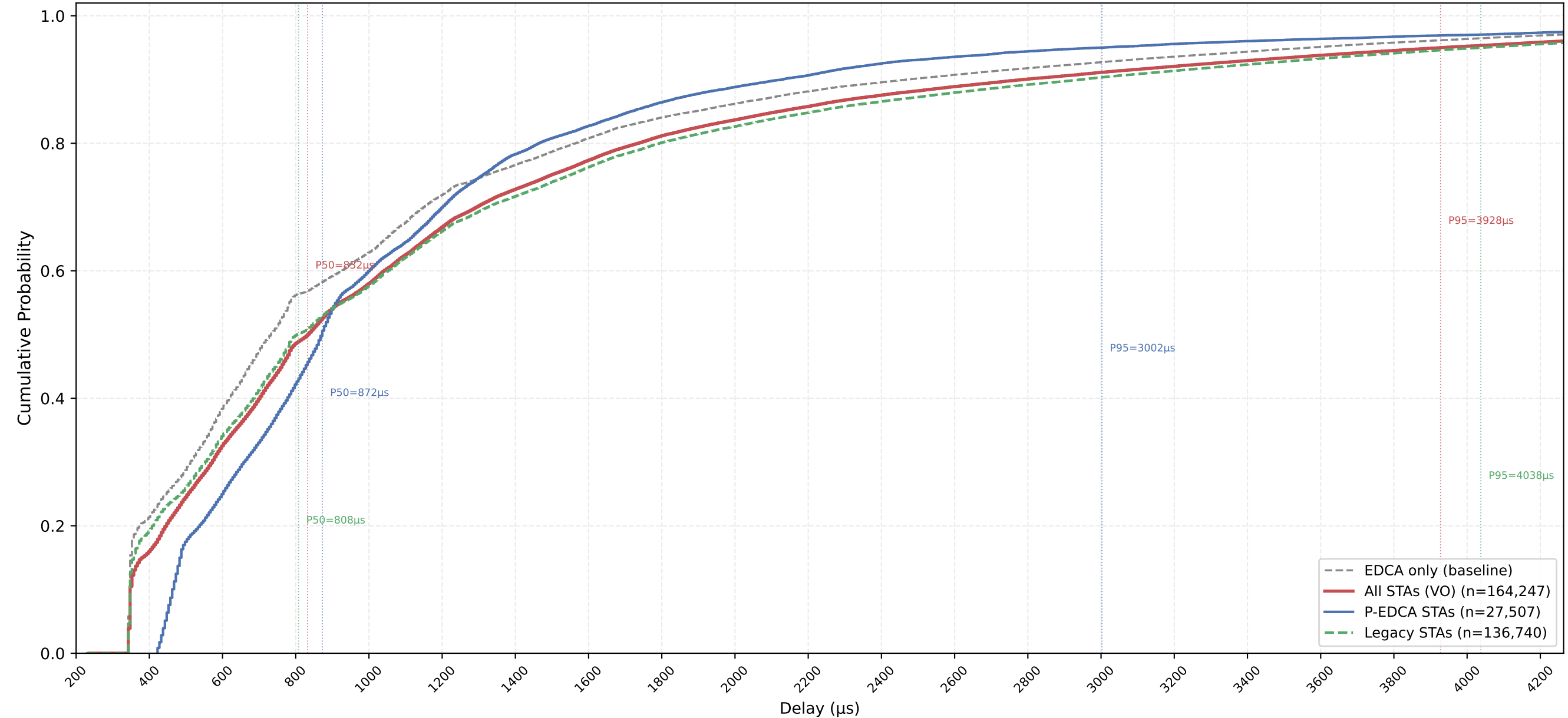
VO Delay CDF — P-EDCA / Legacy / All | CWds=0 × QSRC=0 × PSRC=2 nSta=30, nPedca=5/30, 0.5Mbps, avg of 10 runs
