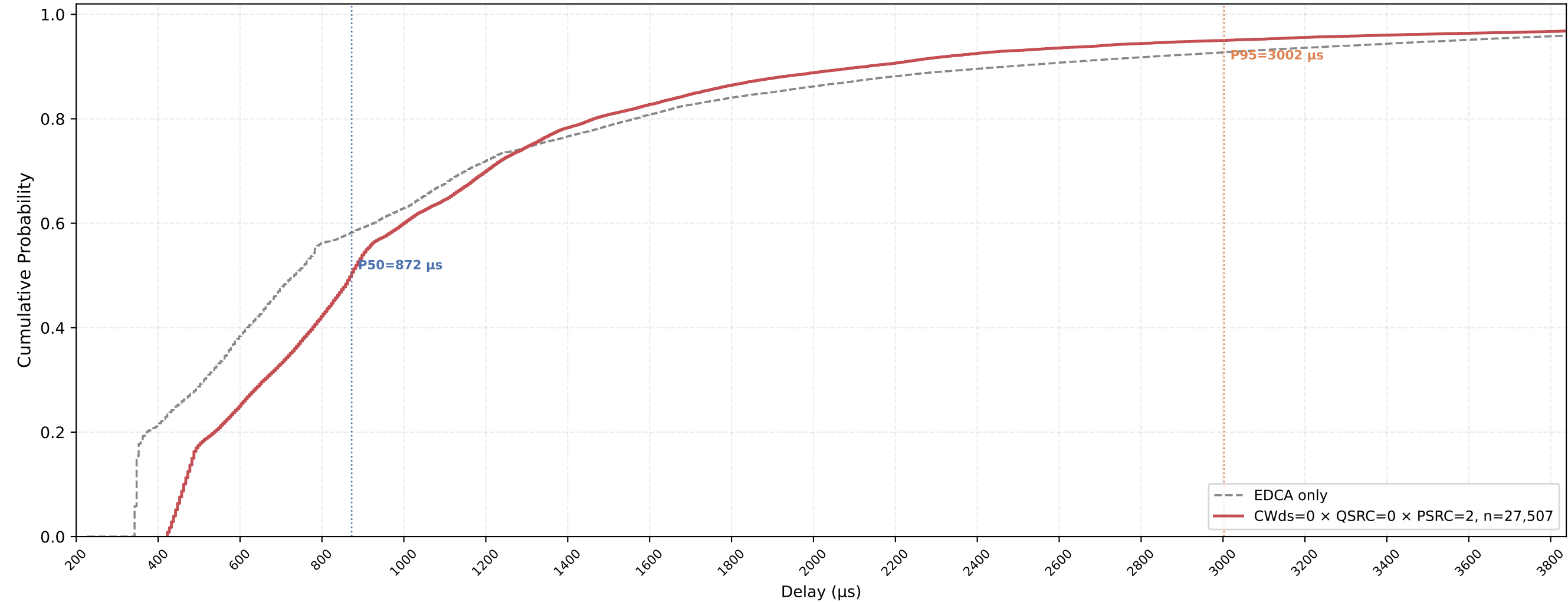
P-EDCA STA VO Delay CDF — CWds=0 × QSRC=0 × PSRC=2 nSta=30, nPedca=5, 0.5Mbps, avg of 10 runs
