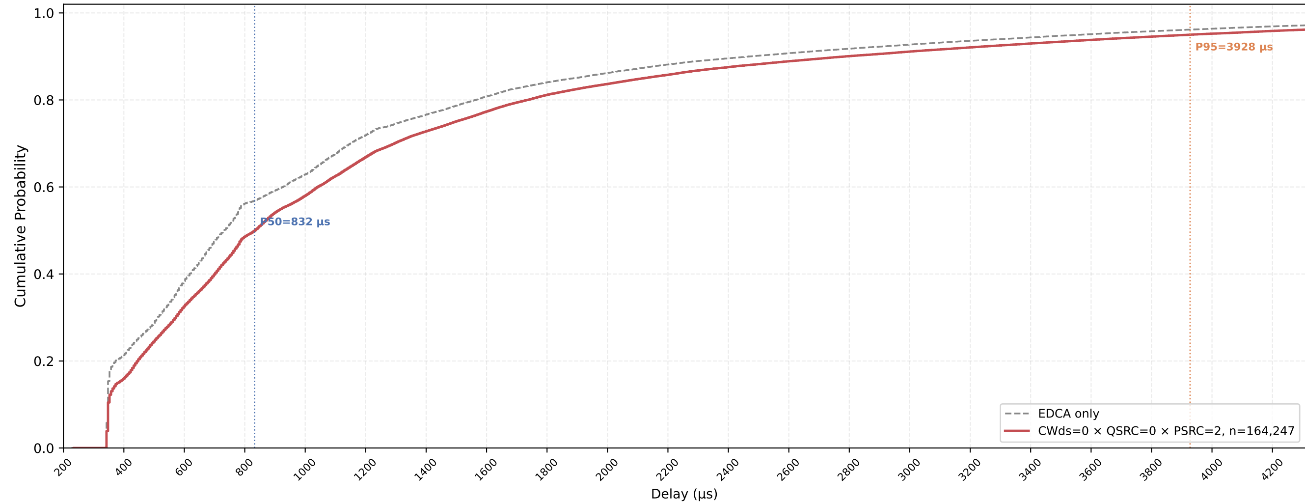
VO (all STAs) Delay CDF — CWds=0 × QSRC=0 × PSRC=2 nSta=30, nPedca=5, 0.5Mbps, avg of 10 runs
