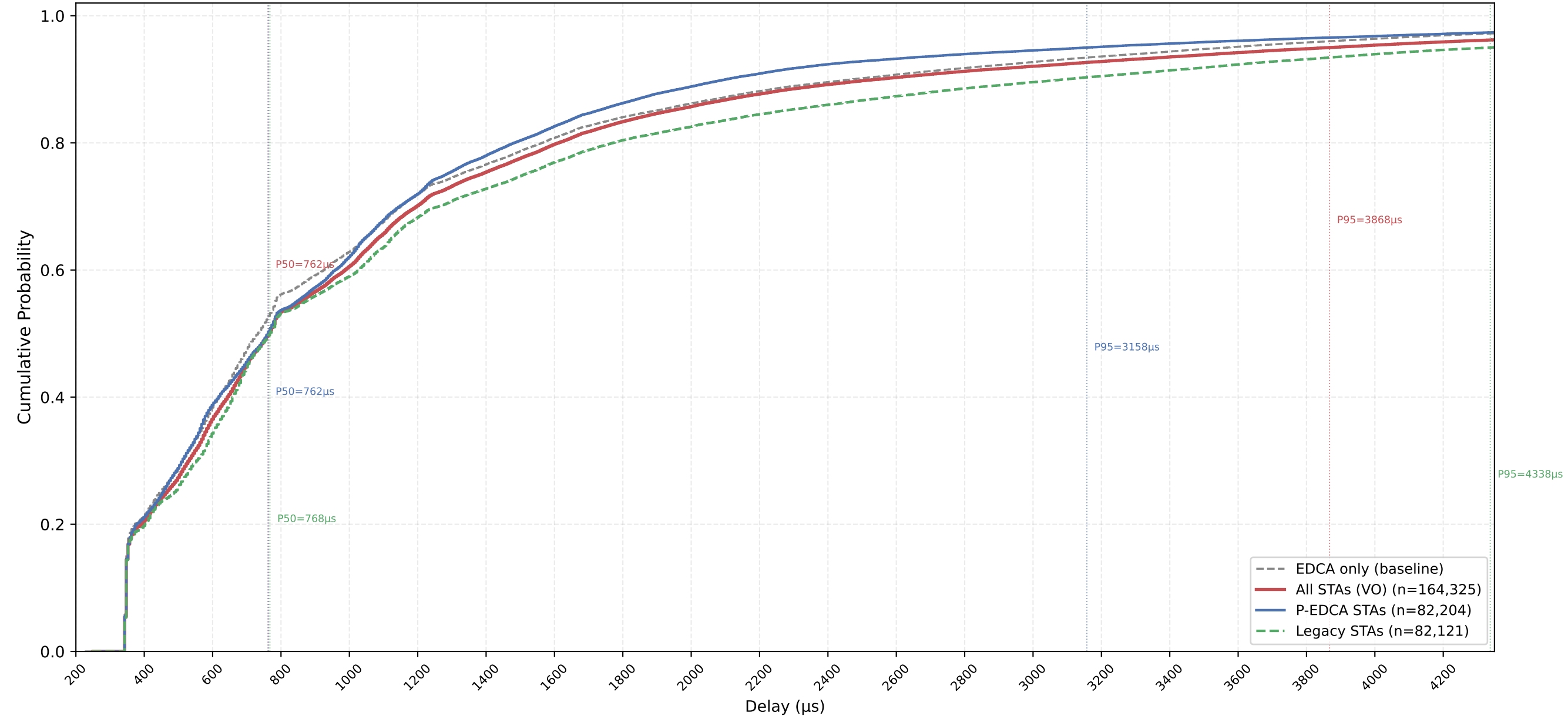
VO Delay CDF — P-EDCA / Legacy / All | CWds=0 × QSRC=1 × PSRC=1 nSta=30, nPedca=15/30, 0.5Mbps, avg of 10 runs
