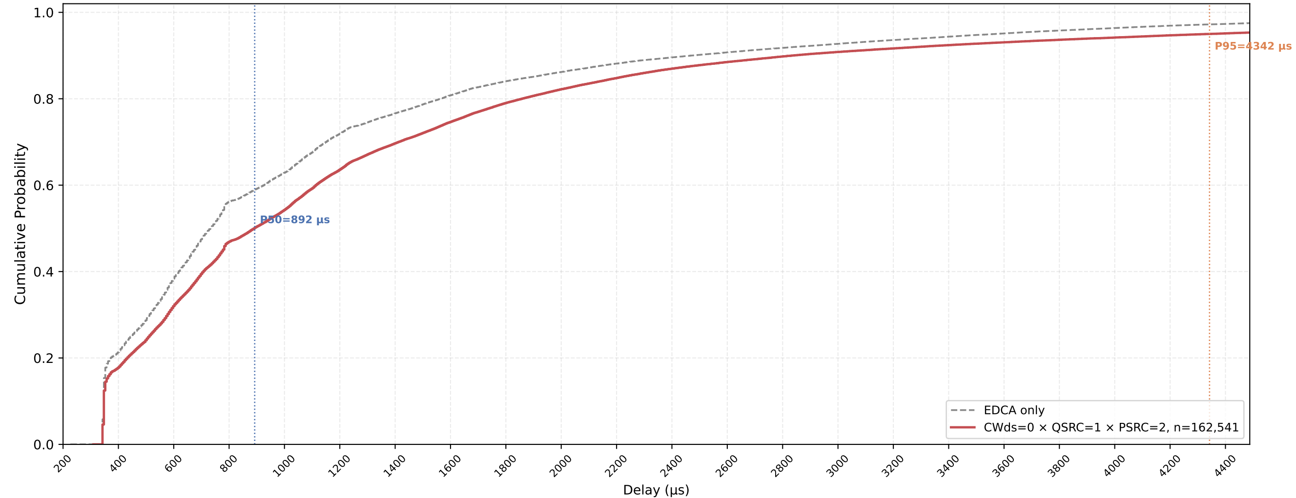
P-EDCA STA VO Delay CDF — CWds=0 × QSRC=1 × PSRC=2 nSta=30, nPedca=30, 0.5Mbps, avg of 10 runs
