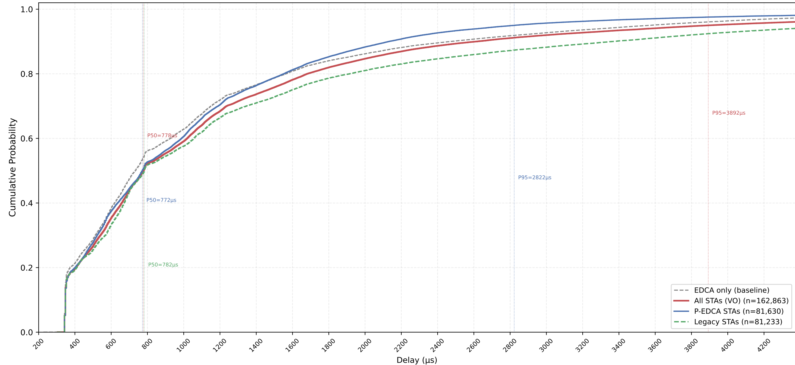
VO Delay CDF — P-EDCA / Legacy / All | CWds=0 × QSRC=1 × PSRC=3 nSta=30, nPedca=15/30, 0.5Mbps, avg of 10 runs
