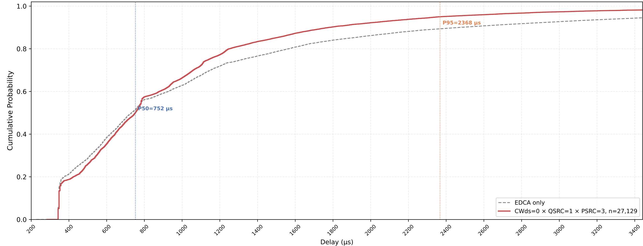
P-EDCA STA VO Delay CDF — CWds=0 × QSRC=1 × PSRC=3 nSta=30, nPedca=5, 0.5Mbps, avg of 10 runs
