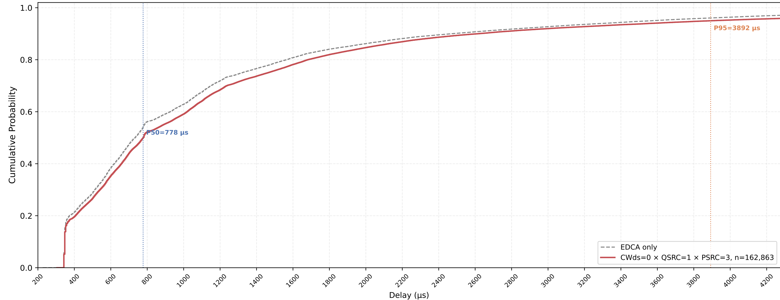
VO (all STAs) Delay CDF — CWds=0 × QSRC=1 × PSRC=3 nSta=30, nPedca=15, 0.5Mbps, avg of 10 runs
