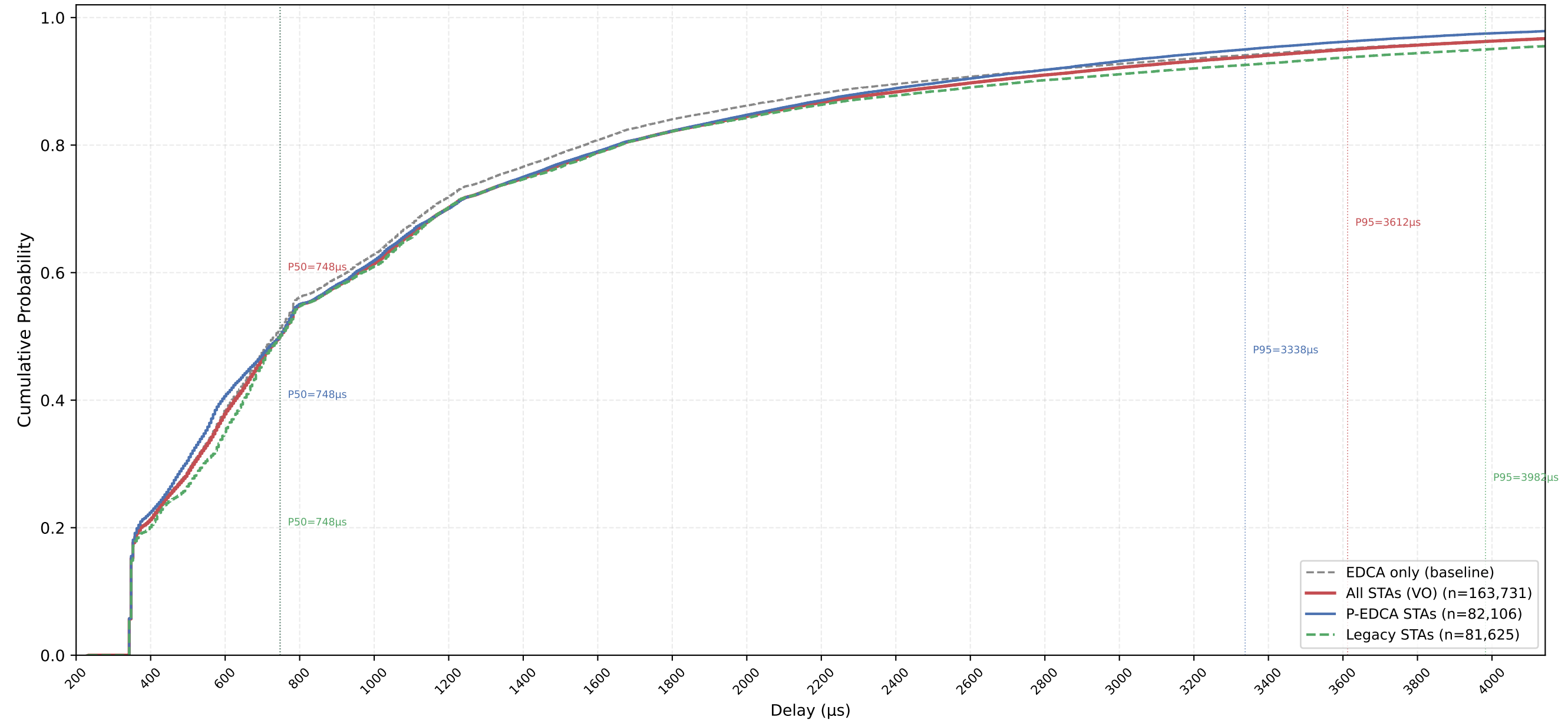
VO Delay CDF — P-EDCA / Legacy / All | CWds=0 × QSRC=2 × PSRC=3 nSta=30, nPedca=15/30, 0.5Mbps, avg of 10 runs
