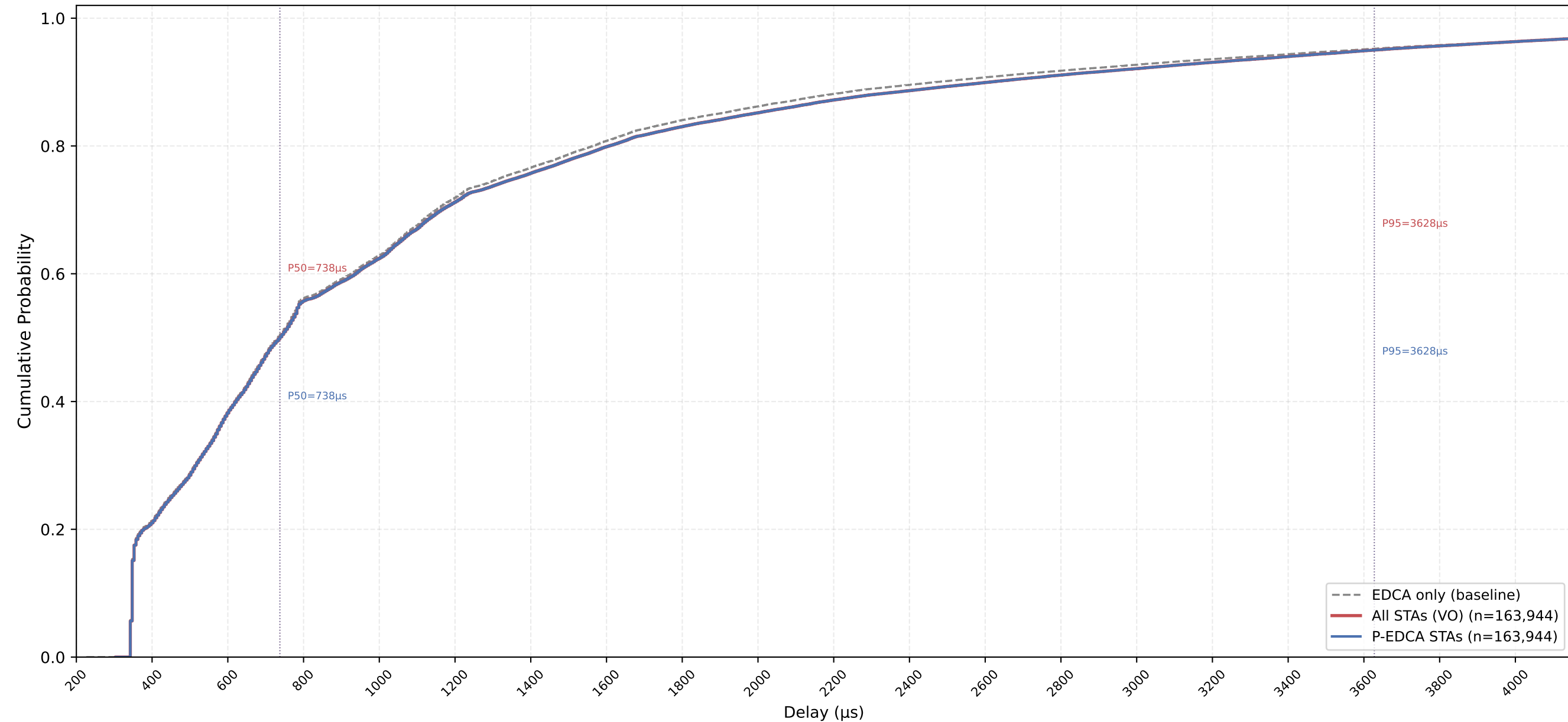
VO Delay CDF — P-EDCA / Legacy / All | CWds=0 × QSRC=3 × PSRC=1 nSta=30, nPedca=30/30, 0.5Mbps, avg of 10 runs
