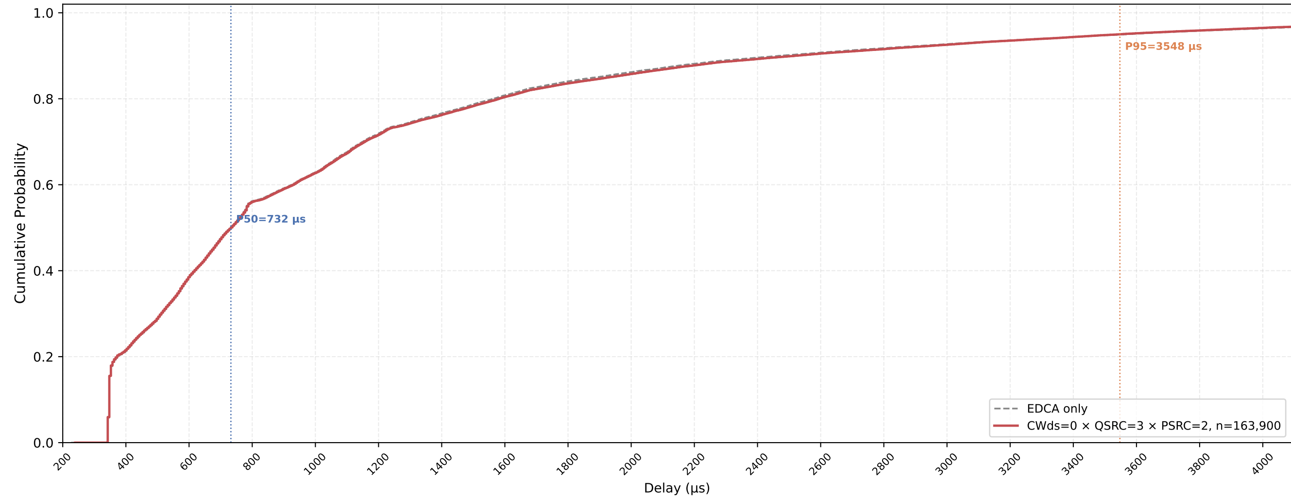
VO (all STAs) Delay CDF — CWds=0 × QSRC=3 × PSRC=2 nSta=30, nPedca=15, 0.5Mbps, avg of 10 runs
