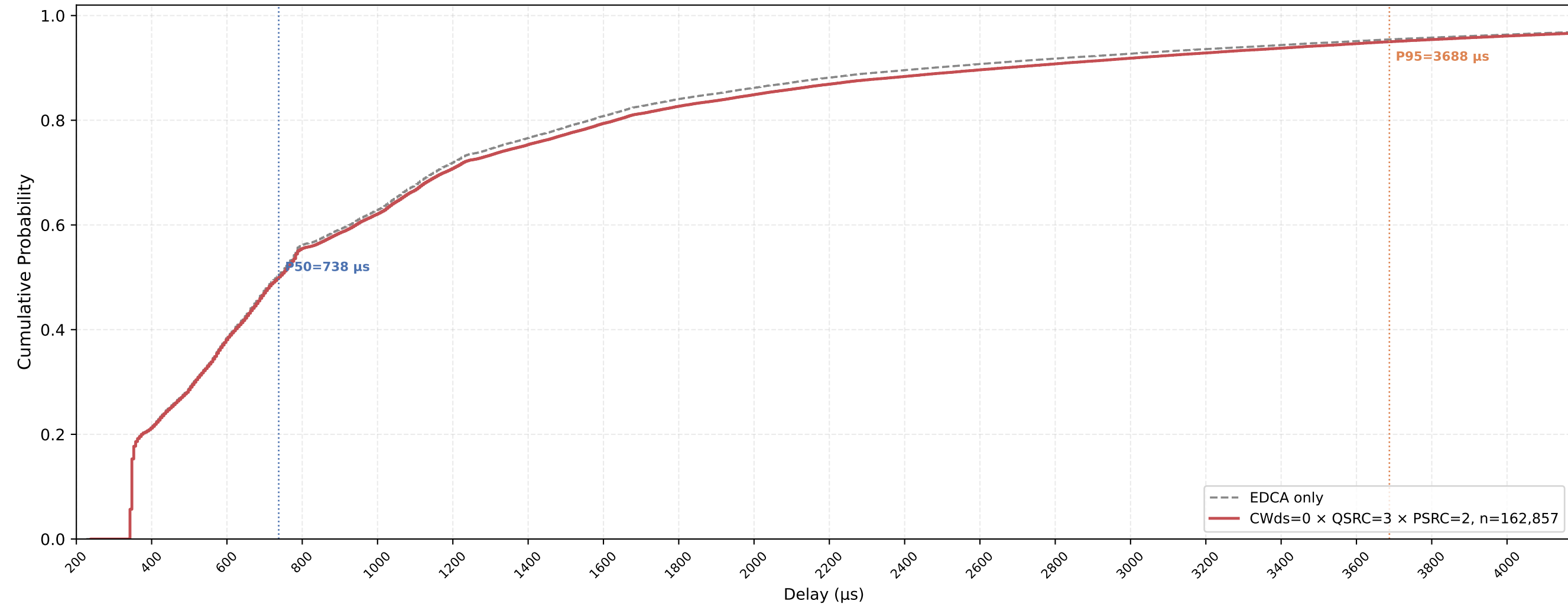
VO (all STAs) Delay CDF — CWds=0 × QSRC=3 × PSRC=2 nSta=30, nPedca=30, 0.5Mbps, avg of 10 runs
