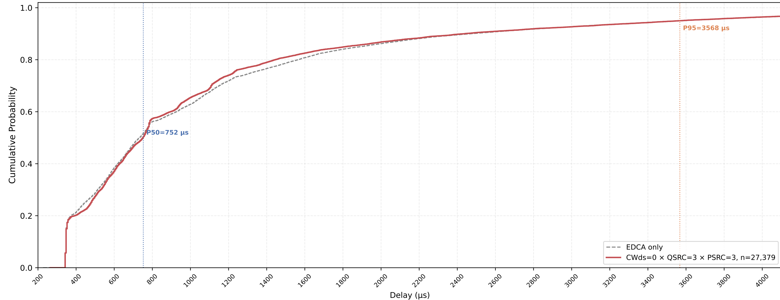
P-EDCA STA VO Delay CDF — CWds=0 × QSRC=3 × PSRC=3 nSta=30, nPedca=5, 0.5Mbps, avg of 10 runs
