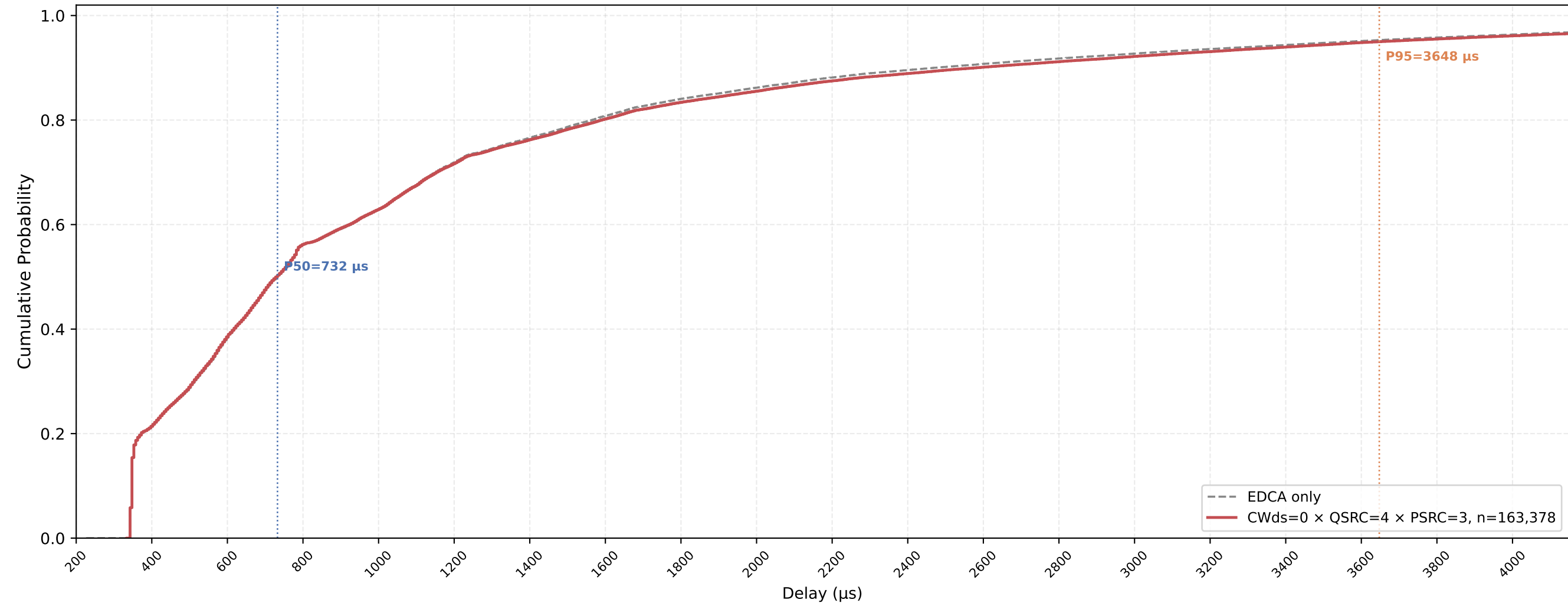
VO (all STAs) Delay CDF — CWds=0 × QSRC=4 × PSRC=3 nSta=30, nPedca=30, 0.5Mbps, avg of 10 runs
