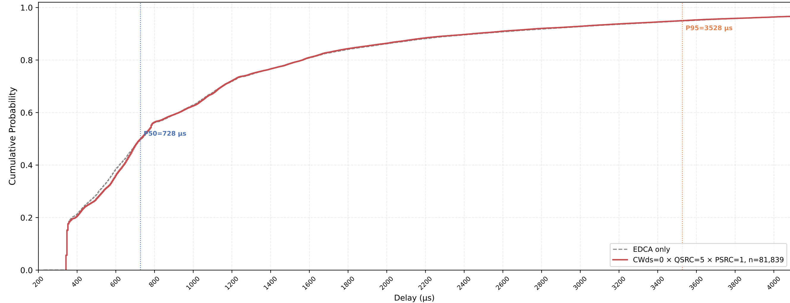
Legacy STA VO Delay CDF — CWds=0 × QSRC=5 × PSRC=1 nSta=30, nPedca=15, 0.5Mbps, avg of 10 runs
