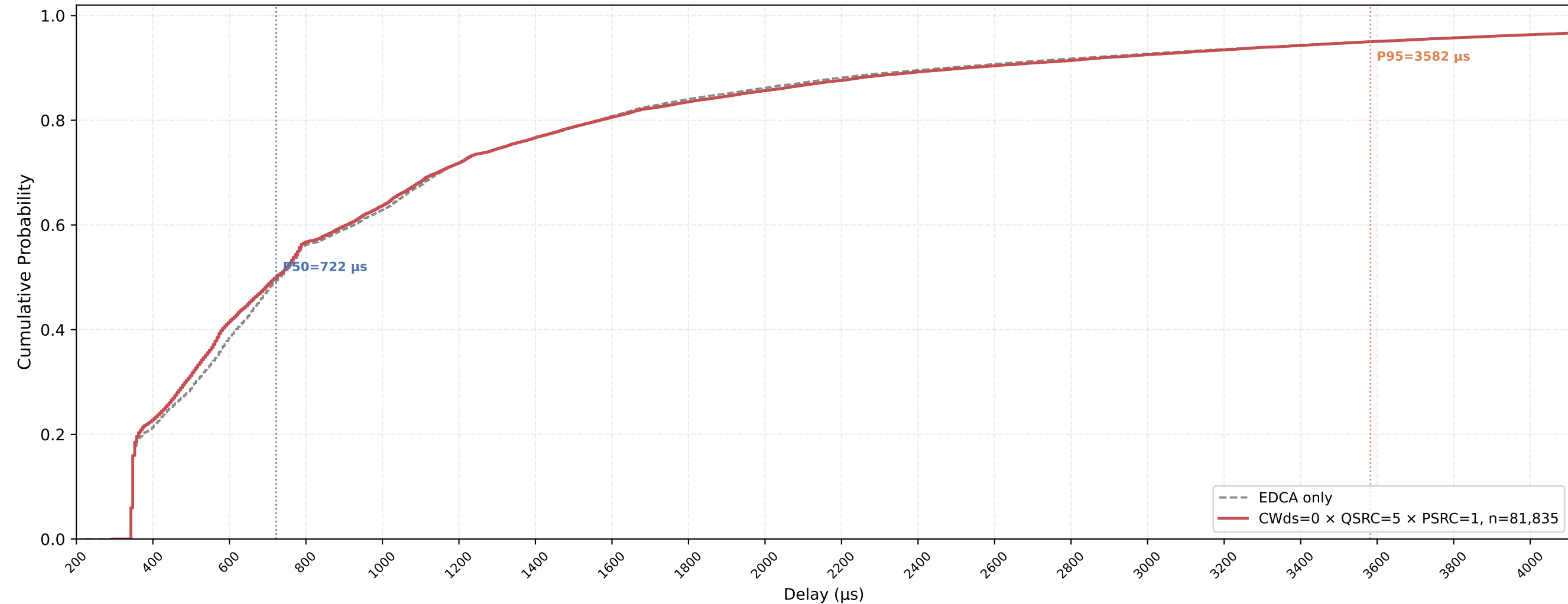
P-EDCA STA VO Delay CDF — CWds=0 × QSRC=5 × PSRC=1 nSta=30, nPedca=15, 0.5Mbps, avg of 10 runs
