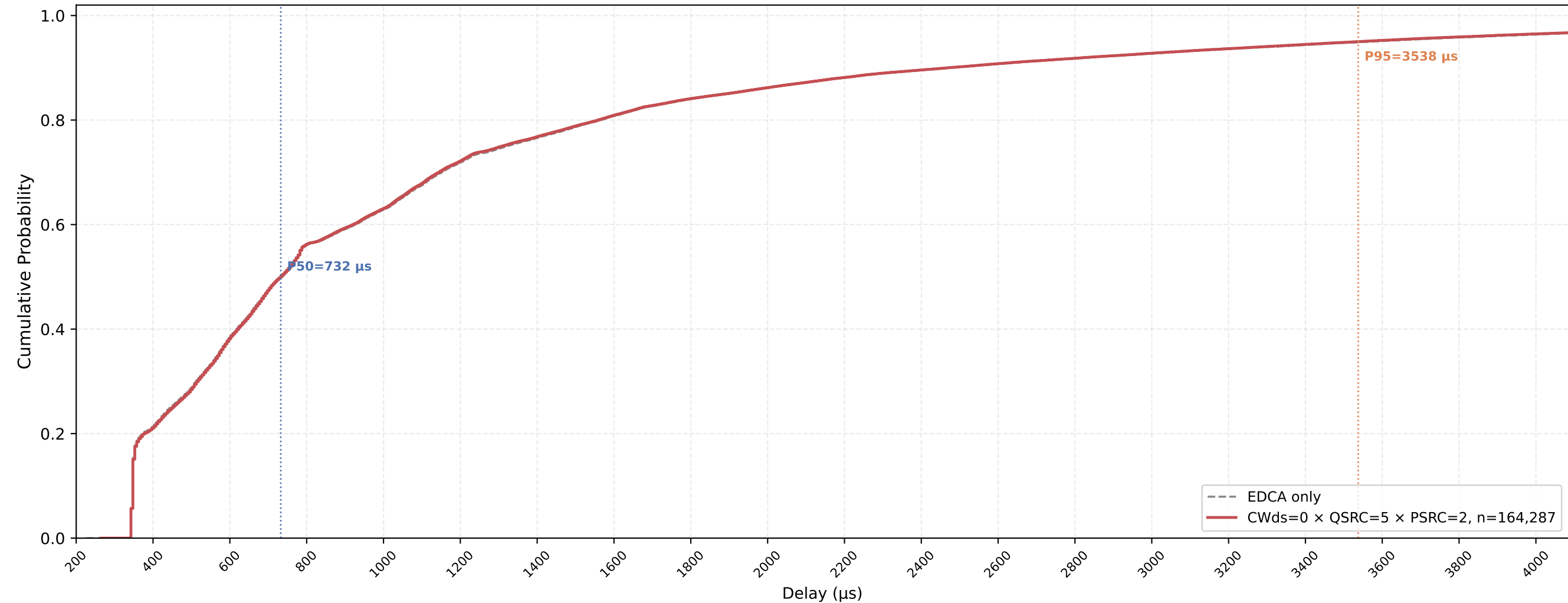
VO (all STAs) Delay CDF — CWds=0 × QSRC=5 × PSRC=2 nSta=30, nPedca=5, 0.5Mbps, avg of 10 runs
