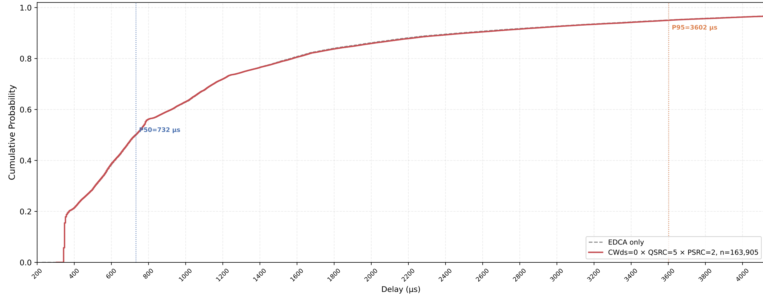
VO (all STAs) Delay CDF — CWds=0 × QSRC=5 × PSRC=2 nSta=30, nPedca=30, 0.5Mbps, avg of 10 runs
