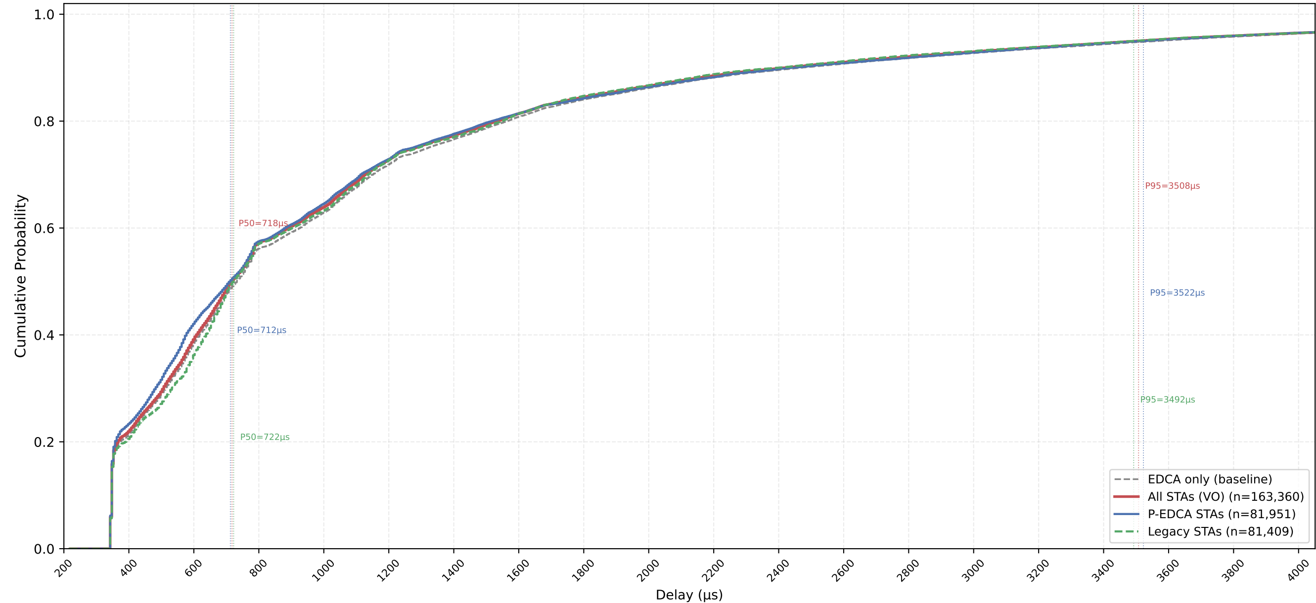
VO Delay CDF — P-EDCA / Legacy / All | CWds=0 × QSRC=5 × PSRC=3 nSta=30, nPedca=15/30, 0.5Mbps, avg of 10 runs
