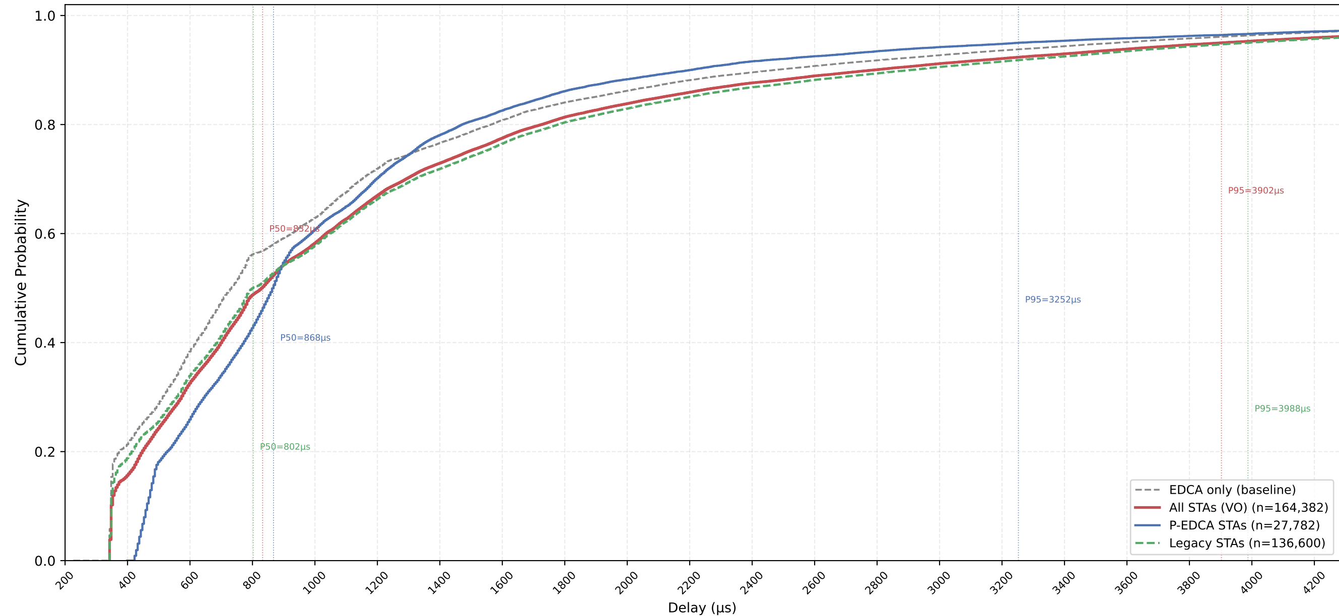
VO Delay CDF — P-EDCA / Legacy / All | CWds=1 × QSRC=0 × PSRC=2 nSta=30, nPedca=5/30, 0.5Mbps, avg of 10 runs
