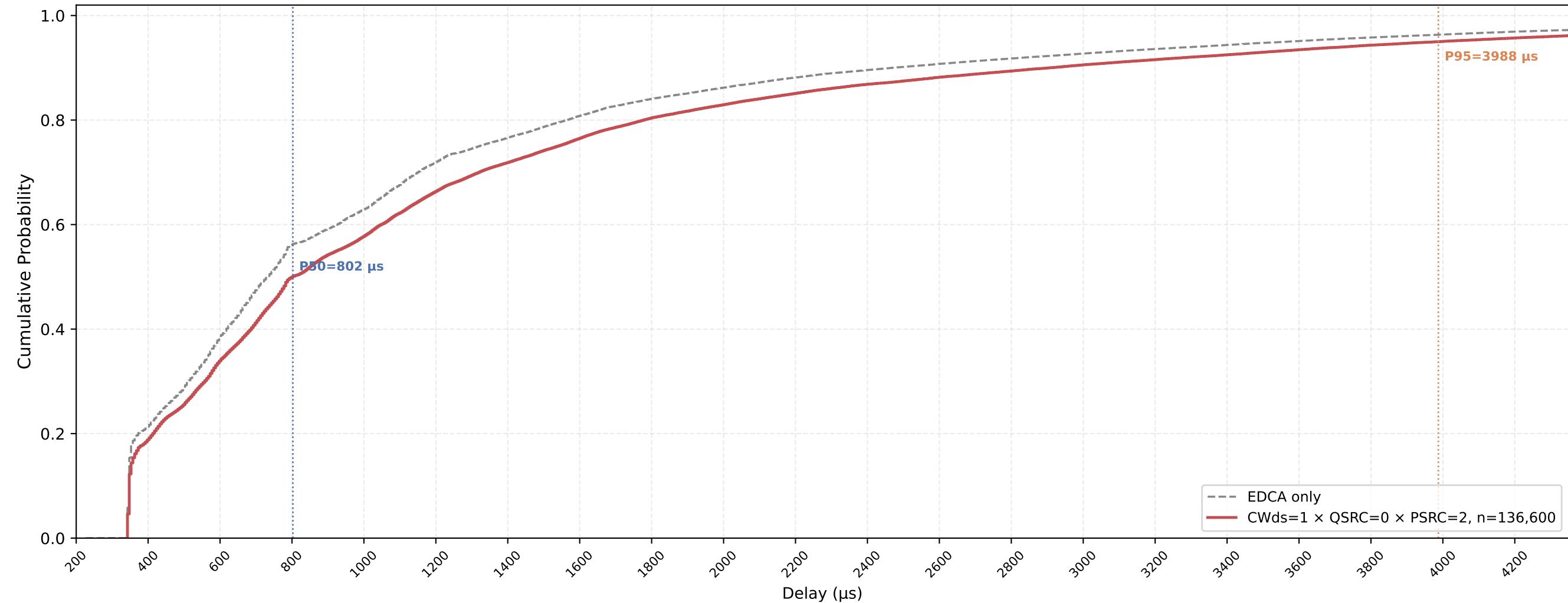
Legacy STA VO Delay CDF — CWds=1 × QSRC=0 × PSRC=2 nSta=30, nPedca=5, 0.5Mbps, avg of 10 runs
