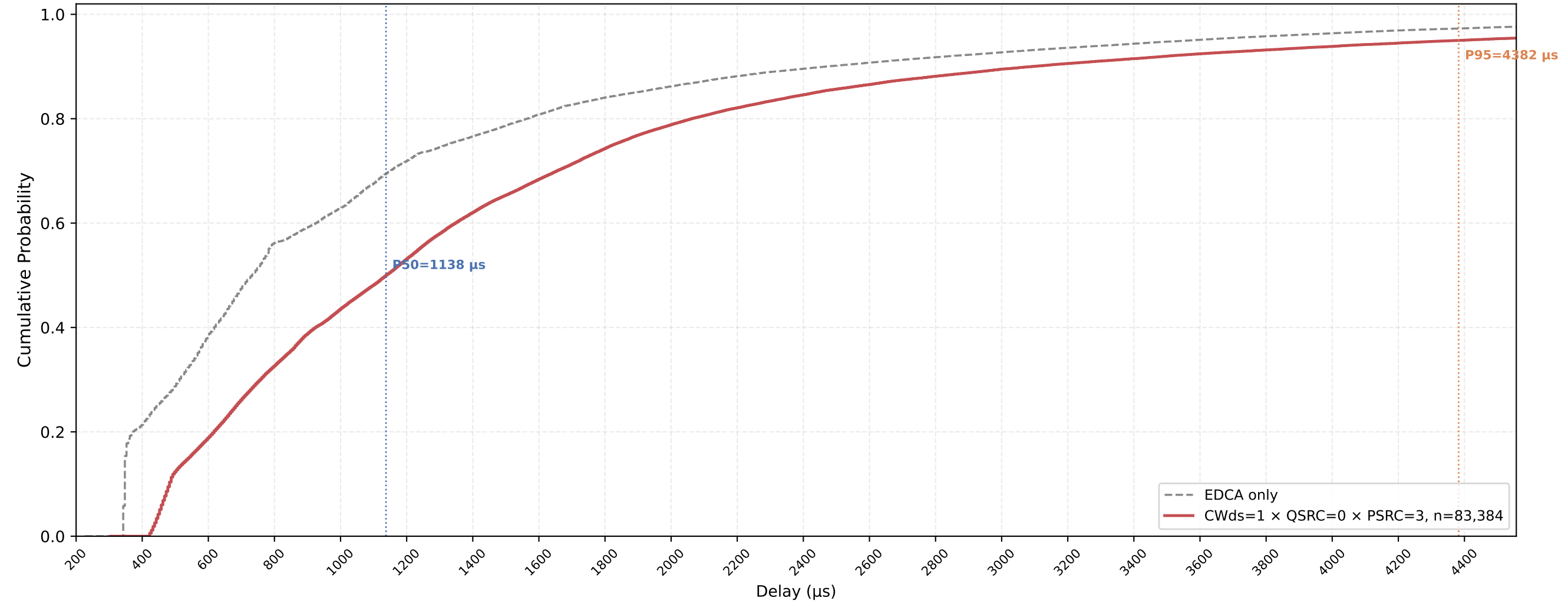
P-EDCA STA VO Delay CDF — CWds=1 × QSRC=0 × PSRC=3 nSta=30, nPedca=15, 0.5Mbps, avg of 10 runs
