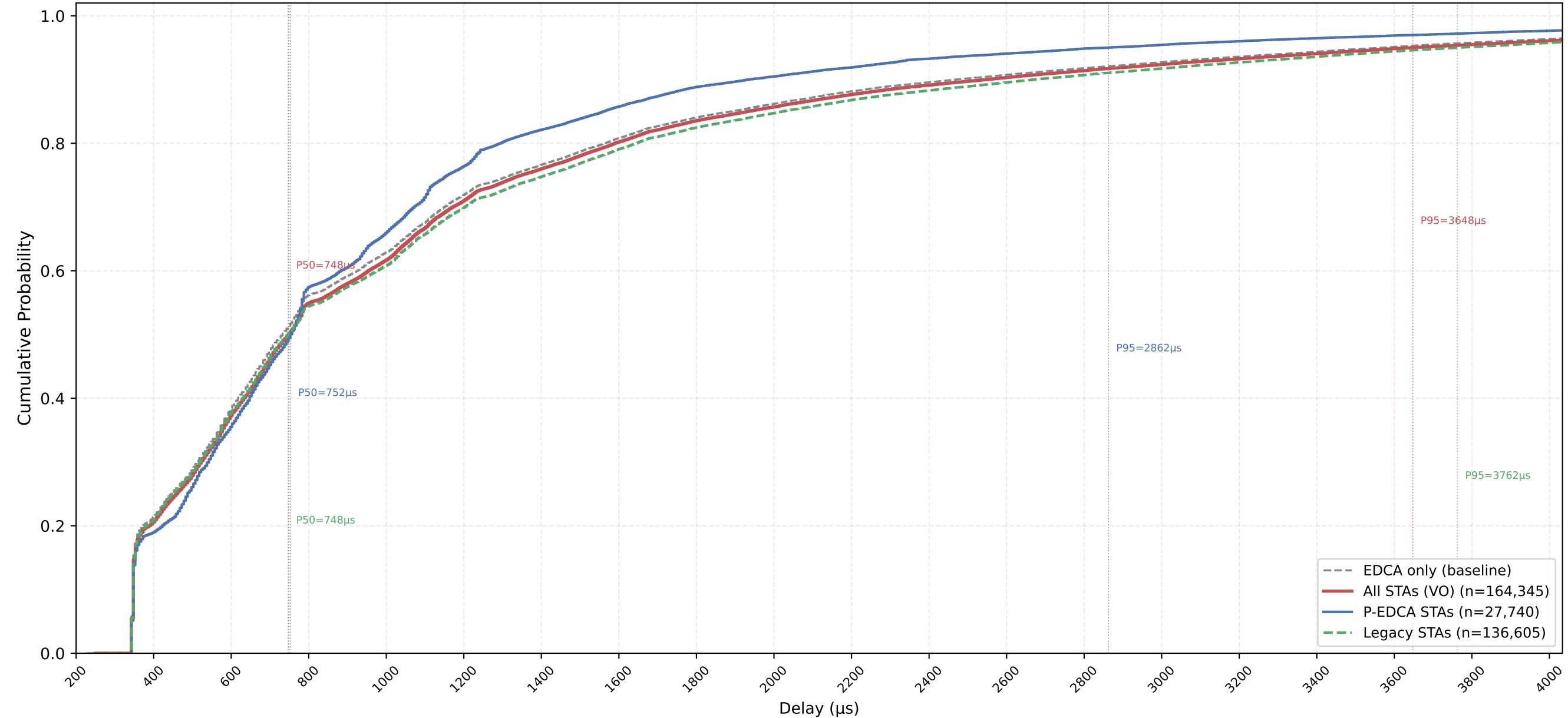
VO Delay CDF — P-EDCA / Legacy / All | CWds=1 × QSRC=1 × PSRC=2 nSta=30, nPedca=5/30, 0.5Mbps, avg of 10 runs
