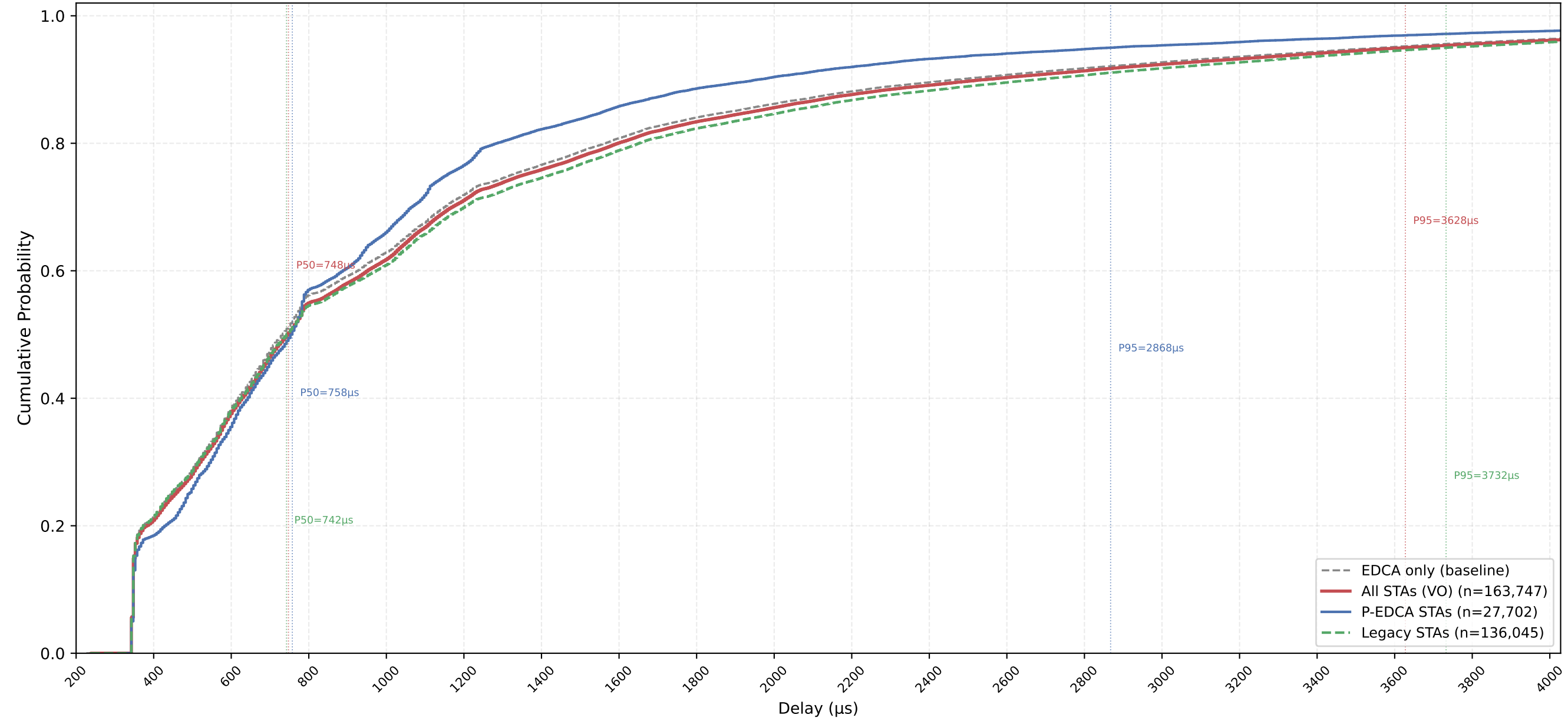
VO Delay CDF — P-EDCA / Legacy / All | CWds=1 × QSRC=1 × PSRC=3 nSta=30, nPedca=5/30, 0.5Mbps, avg of 10 runs
