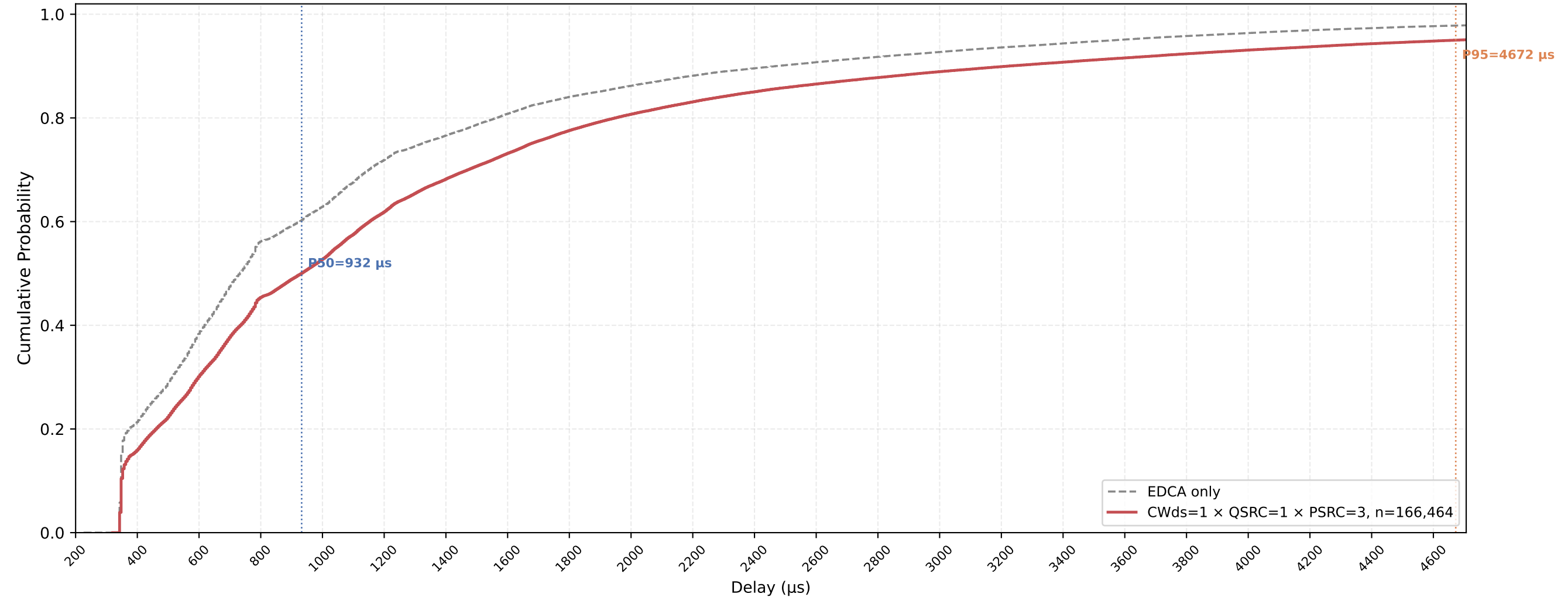
P-EDCA STA VO Delay CDF — CWds=1 × QSRC=1 × PSRC=3 nSta=30, nPedca=30, 0.5Mbps, avg of 10 runs
