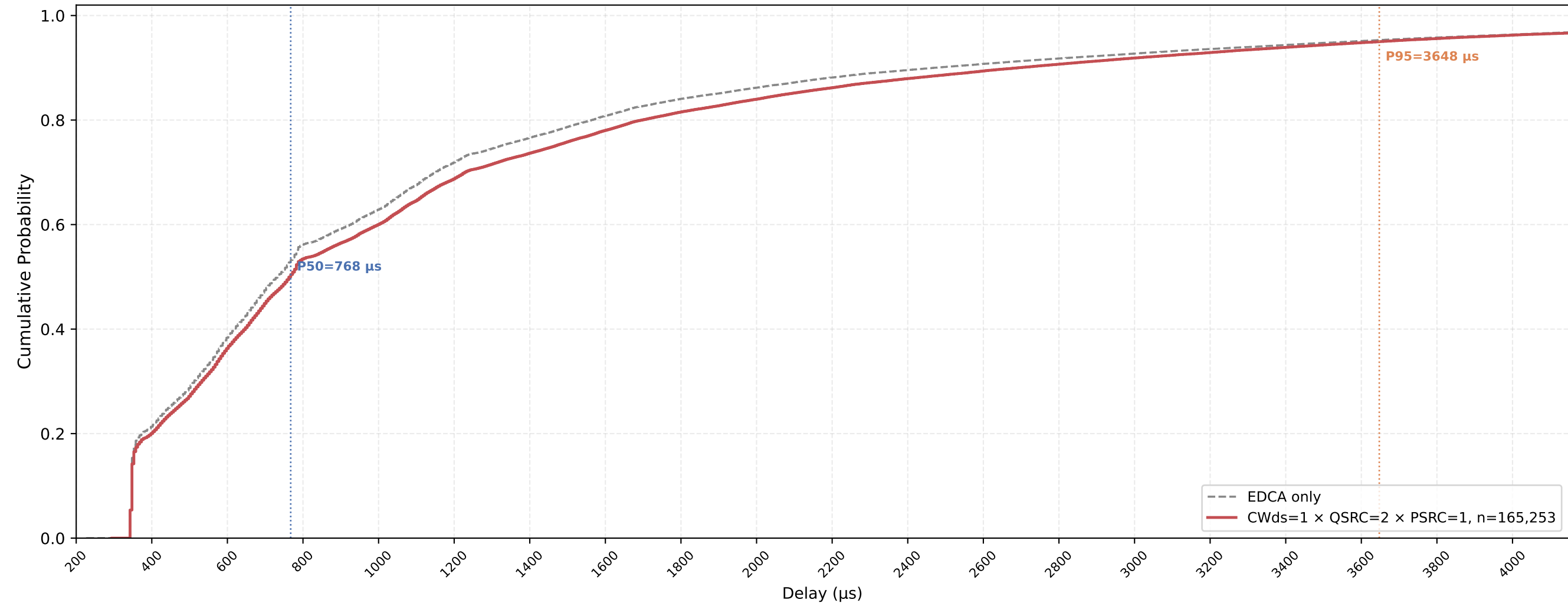
VO (all STAs) Delay CDF — CWds=1 × QSRC=2 × PSRC=1 nSta=30, nPedca=30, 0.5Mbps, avg of 10 runs
