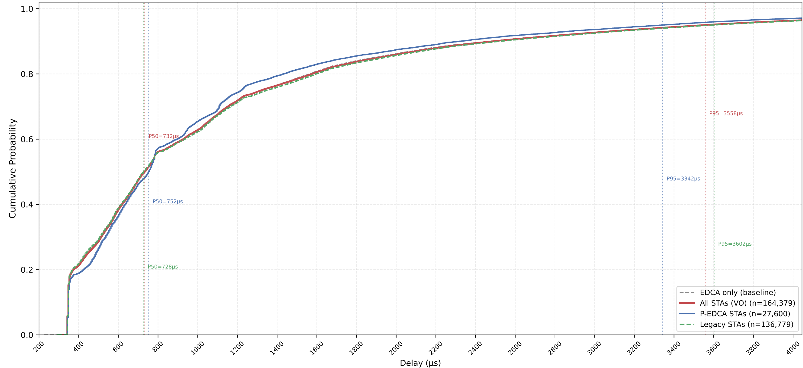
VO Delay CDF — P-EDCA / Legacy / All | CWds=1 × QSRC=2 × PSRC=2 nSta=30, nPedca=5/30, 0.5Mbps, avg of 10 runs
