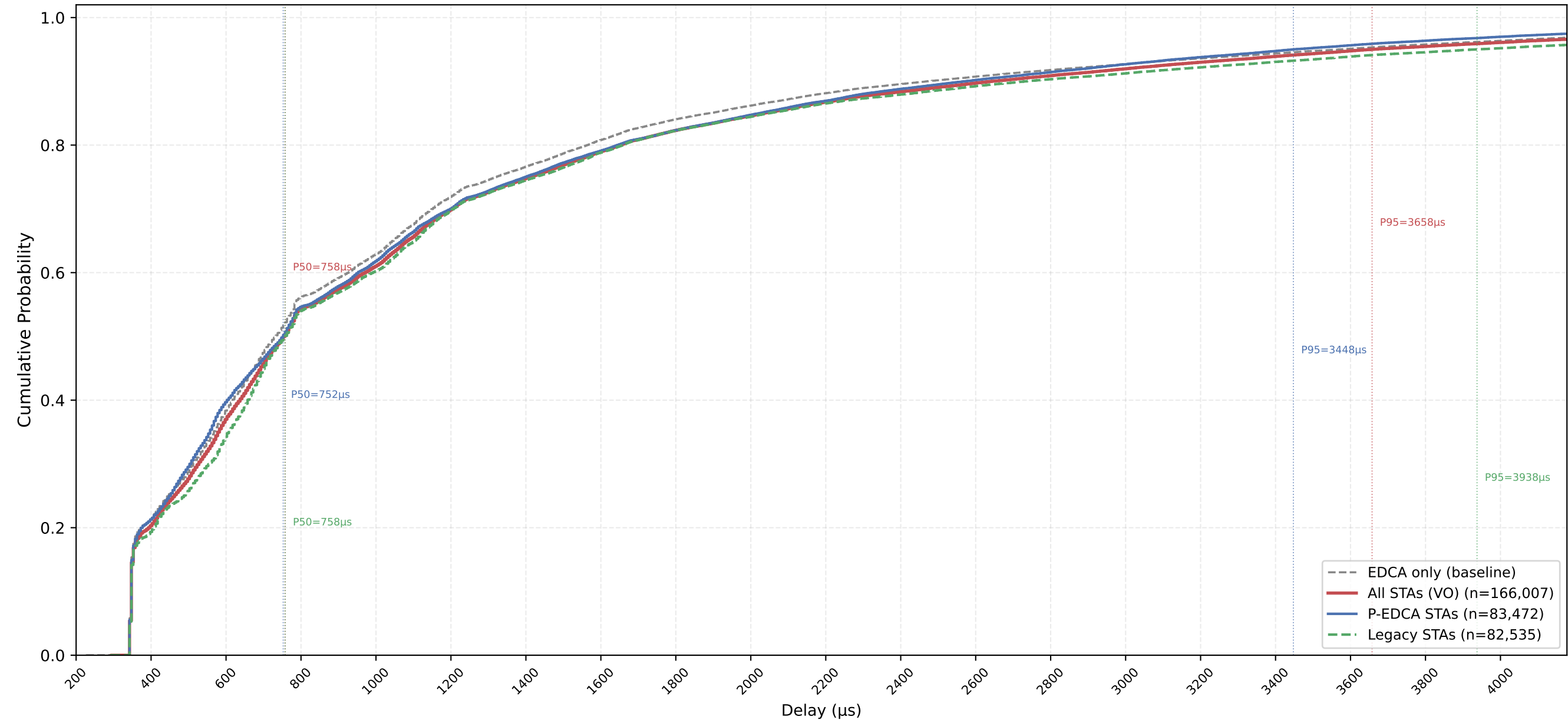
VO Delay CDF — P-EDCA / Legacy / All | CWds=1 × QSRC=2 × PSRC=3 nSta=30, nPedca=15/30, 0.5Mbps, avg of 10 runs
