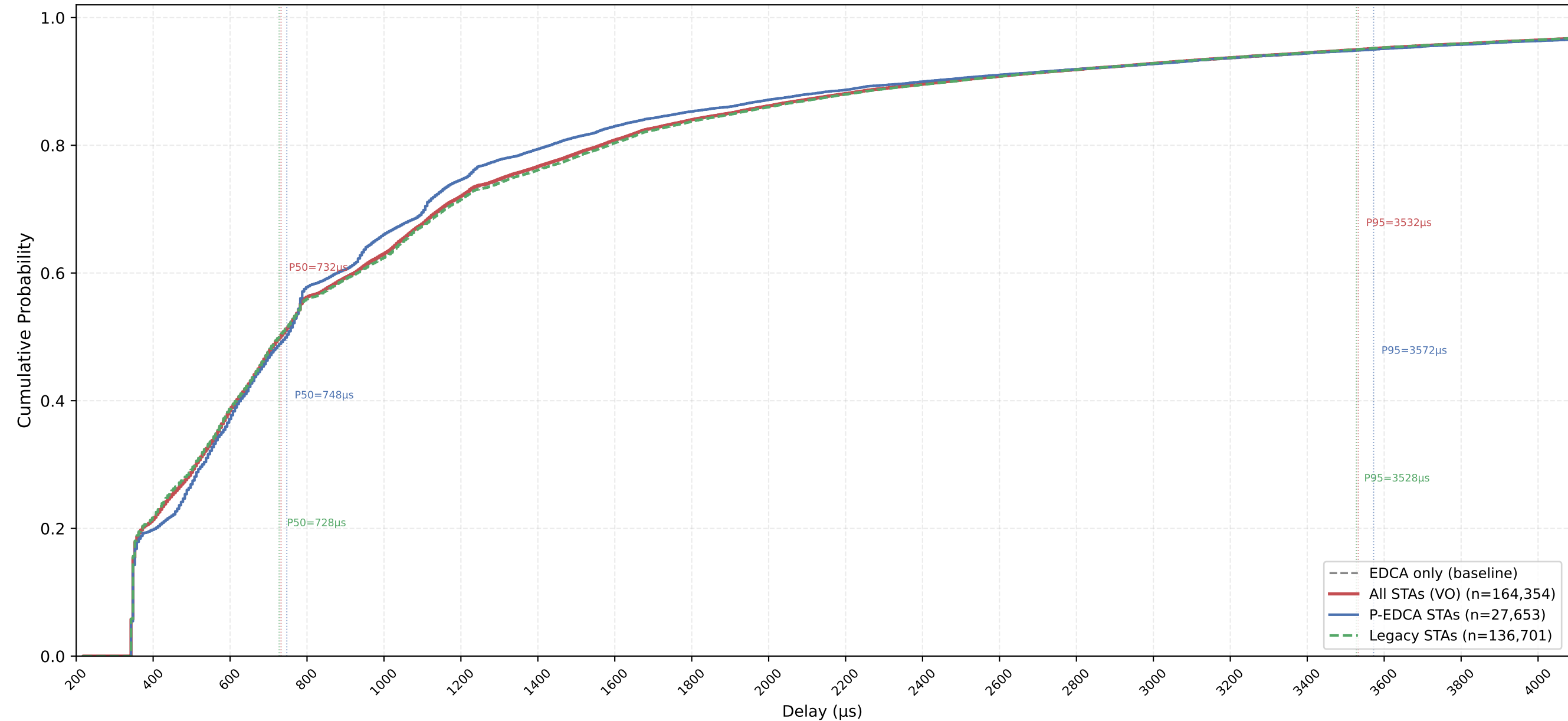
VO Delay CDF — P-EDCA / Legacy / All | CWds=1 × QSRC=3 × PSRC=1 nSta=30, nPedca=5/30, 0.5Mbps, avg of 10 runs
